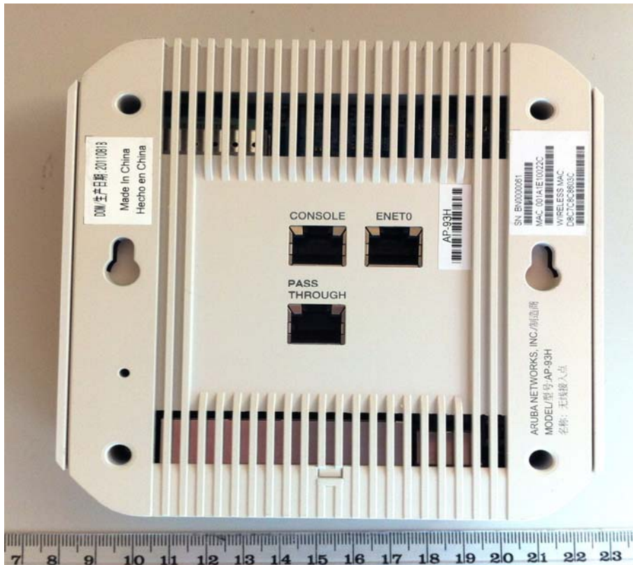
Photo 2 – Bottom View
