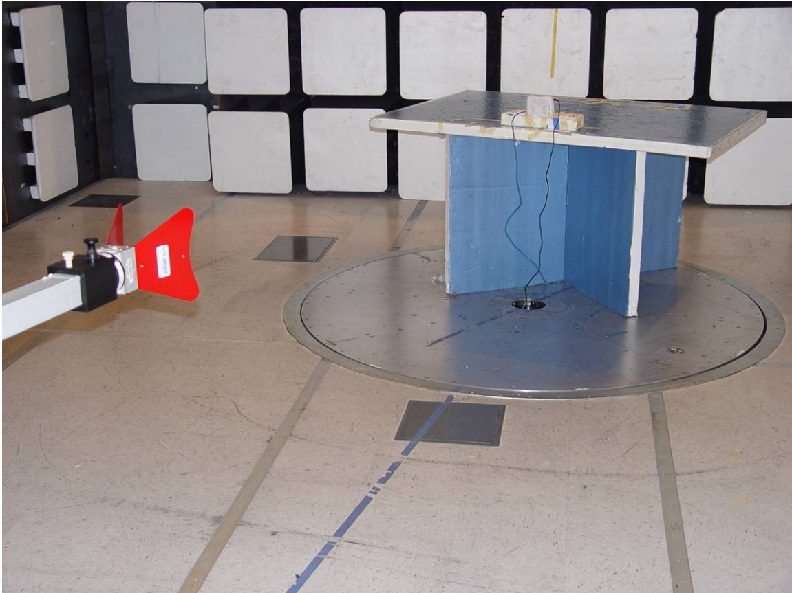
AP-93; Radiated Emissions > 1GHz
