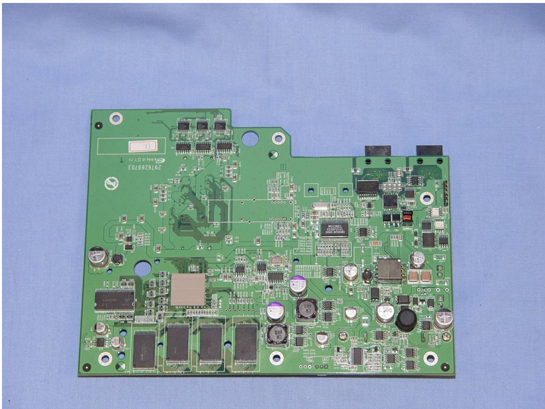
Motherboard assembly bottom
