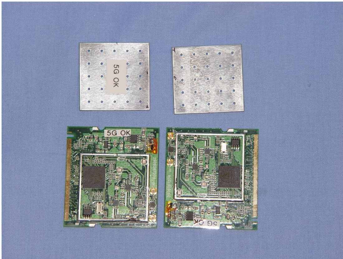
RF assemblies top
