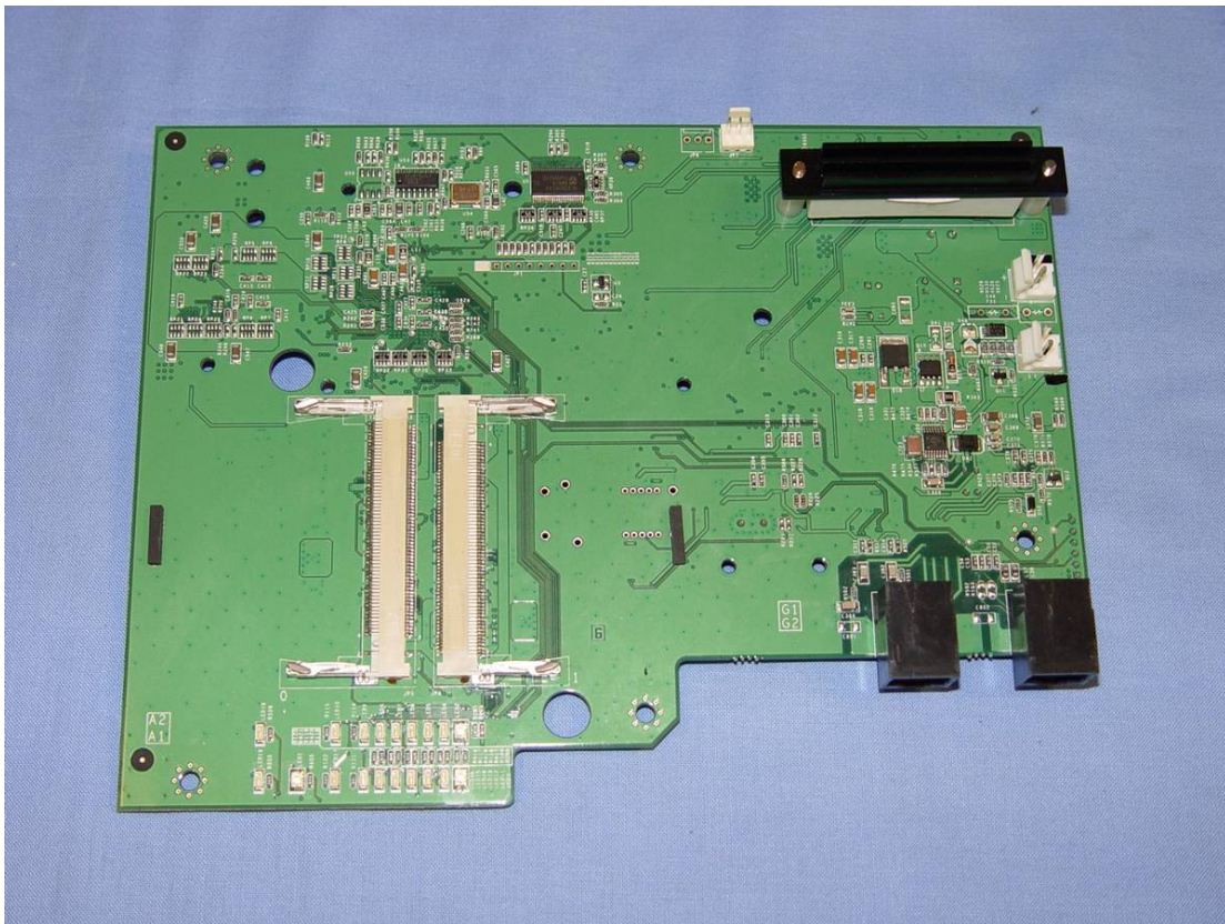
Motherboard top with RF assemblies removed
