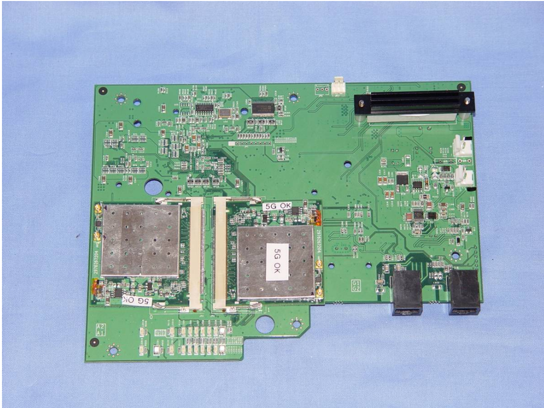
Motherboard top with RF assemblies
