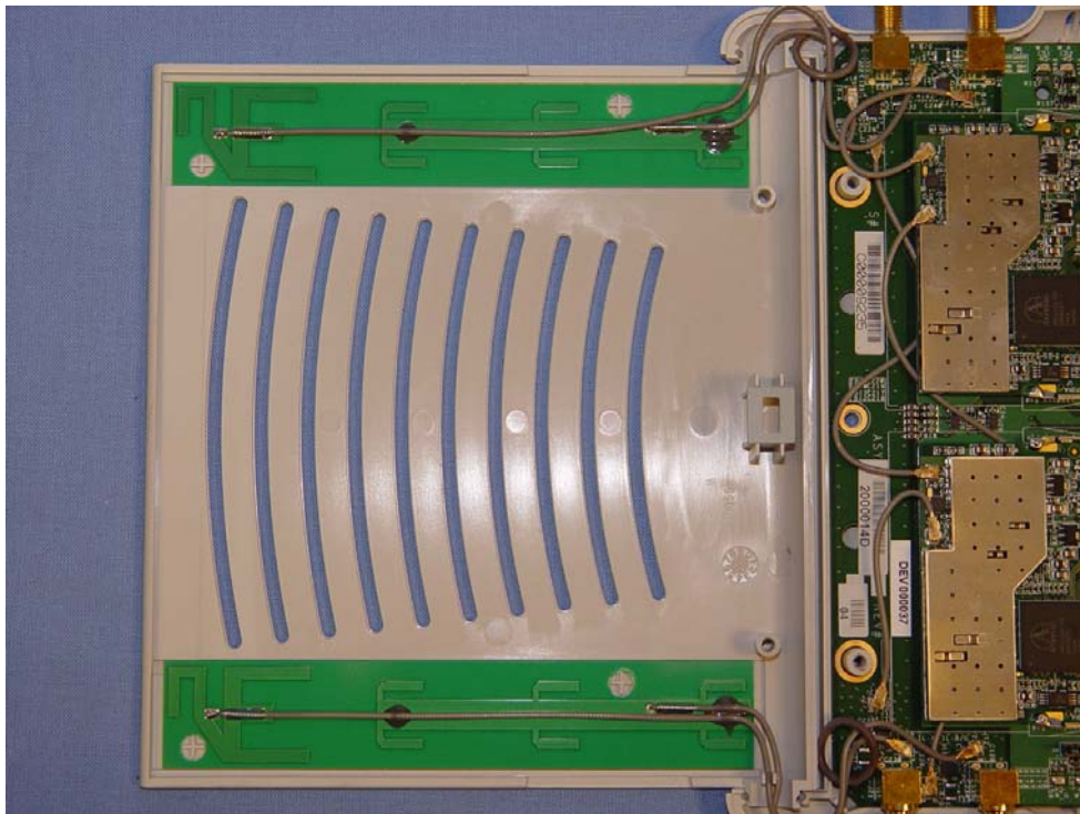
Antennas front
