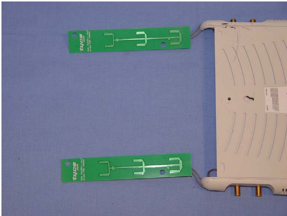
Antennas rear
