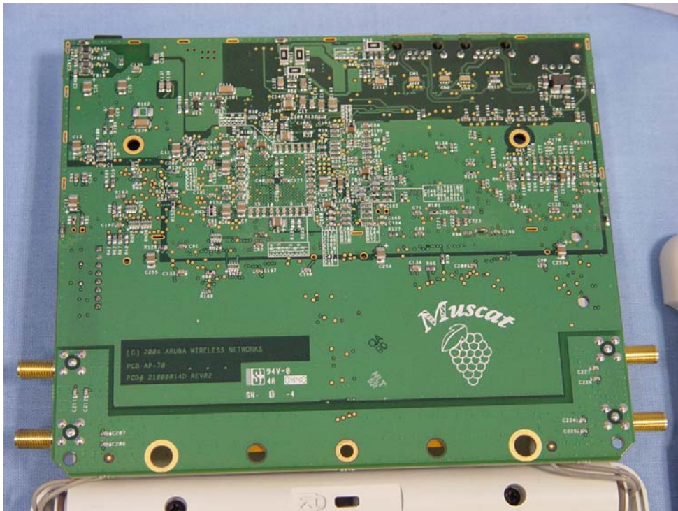
Motherboard rear
