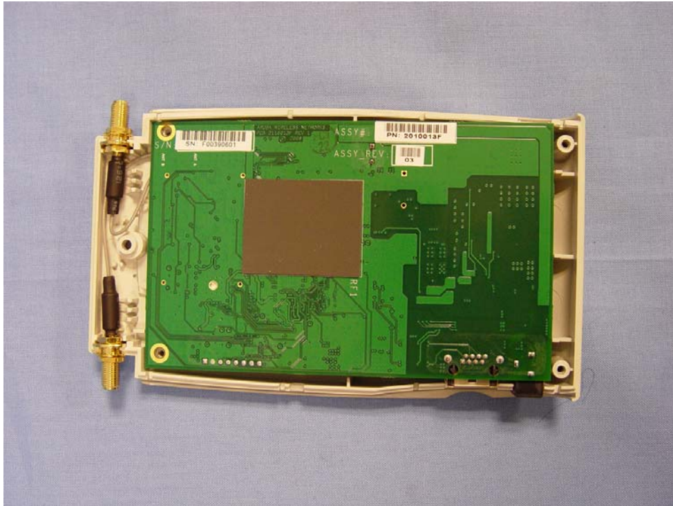
AP 60 Motherboard rear
