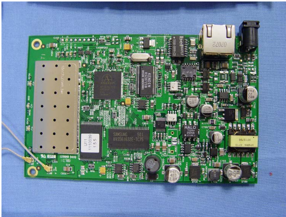
AP 61 Motherboard front
