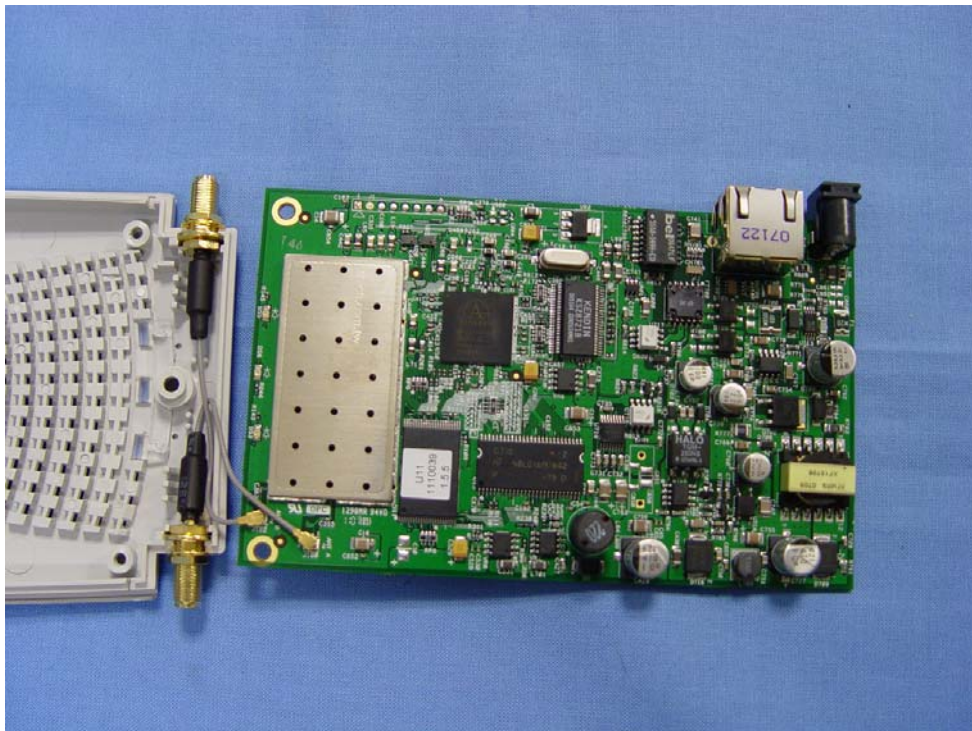
AP 60 Motherboard front
