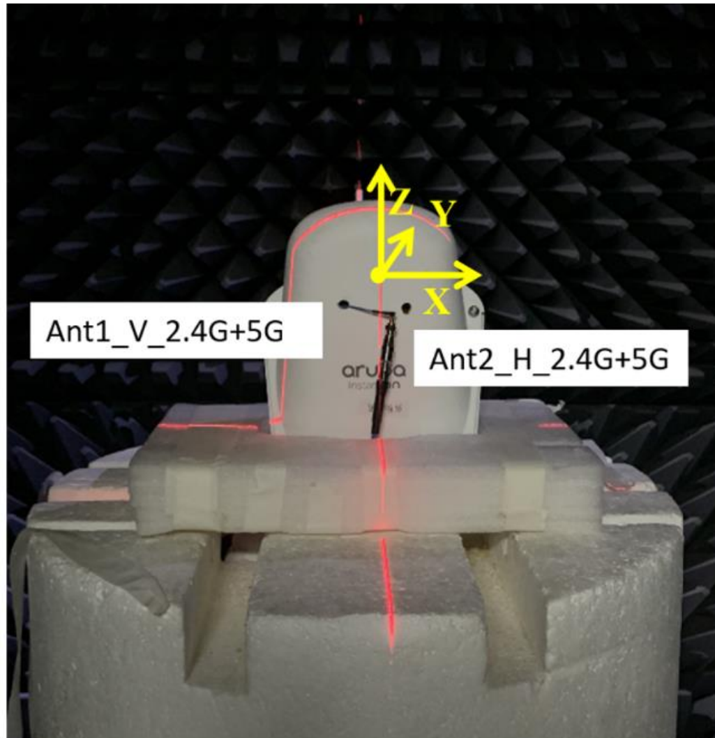
Measurement setup
