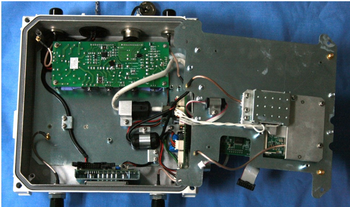
Picture 2 – Assembly, main Board open
