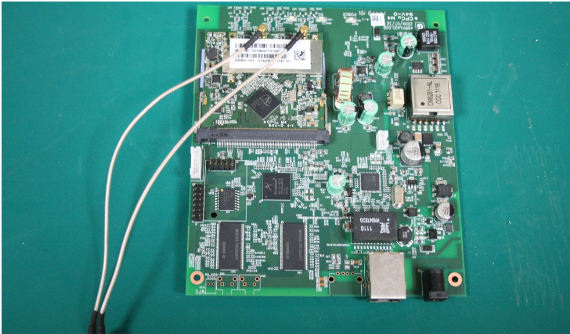
Picture 5 – Main PCB Board (Radio Card 1 shown)
