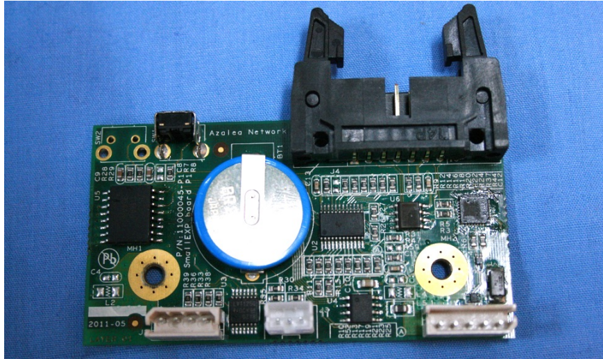
Picture 9 – Small EXP Board – Top
