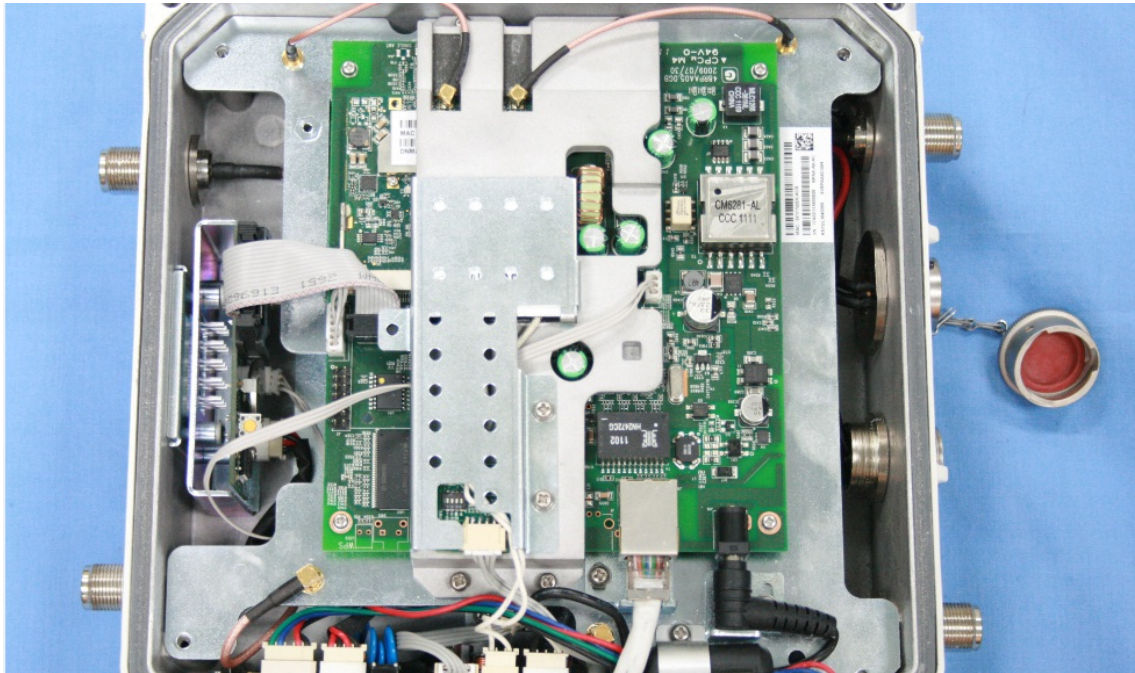
Picture 1 – Assembly
