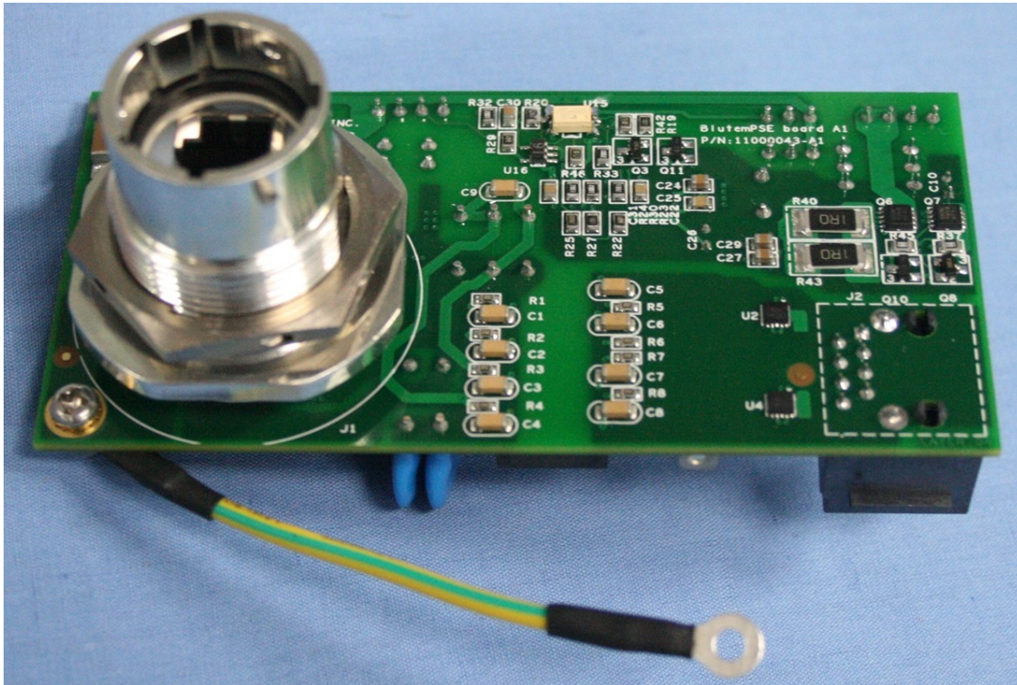
Picture 4 – PSE Board Back
