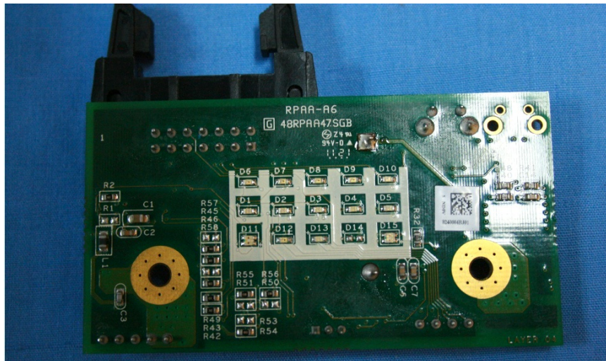
Picture 10 – Small EXP Board – Back
