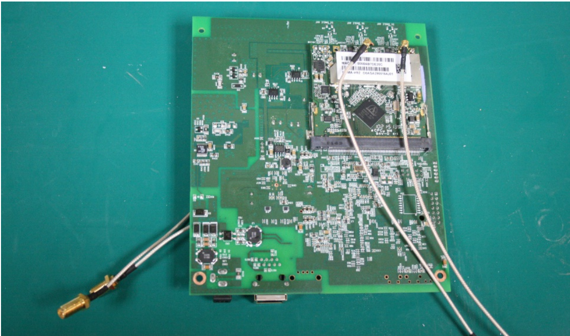
Picture 6 – Main PCB Board (Radio Card 2 shown)
