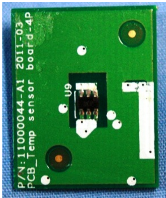
Picture 12 – Temp Sensor Board – Back
