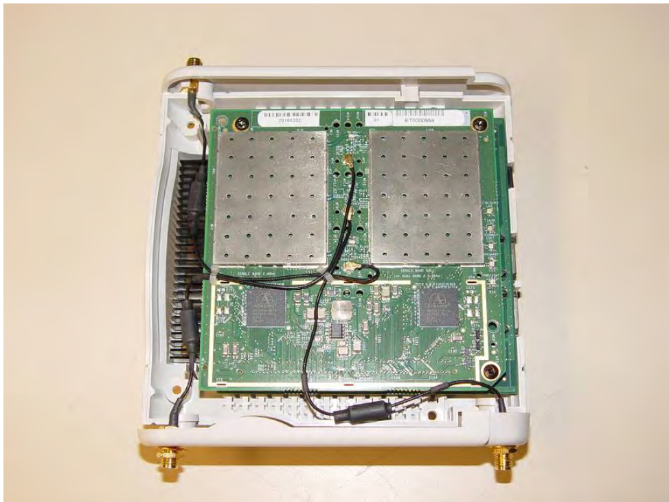
AP124 Internal View
