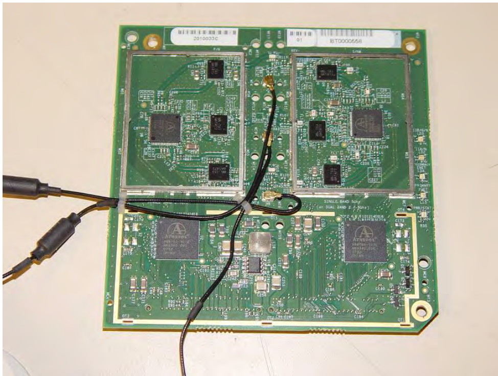
AP125 RF Assembly Front
