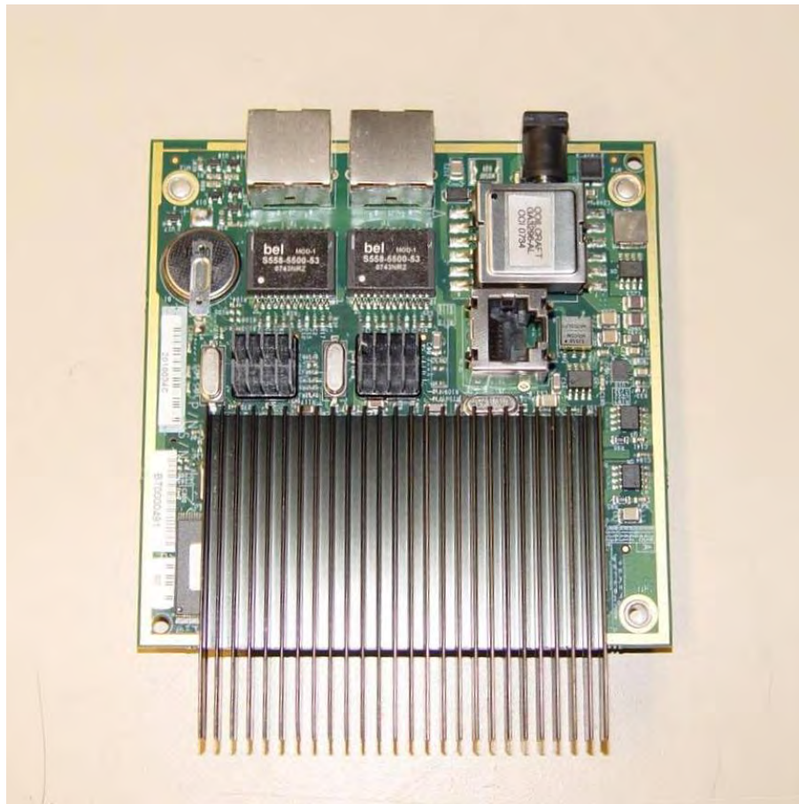
AP124 Motherboard Front
