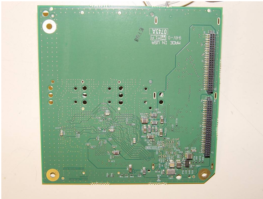
AP121 RF Assembly Bottom
