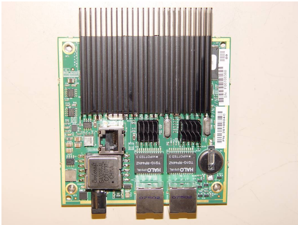
AP121 Motherboard Top
