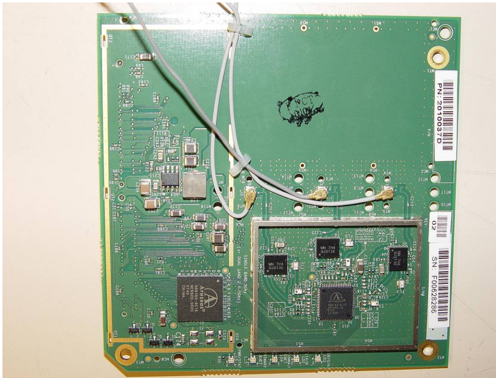
AP120 RF Assembly Top
