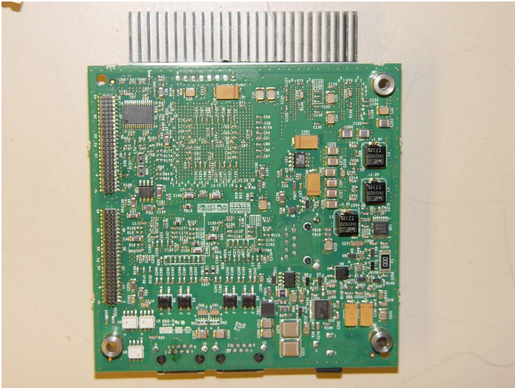
AP120 Motherboard Bottom
