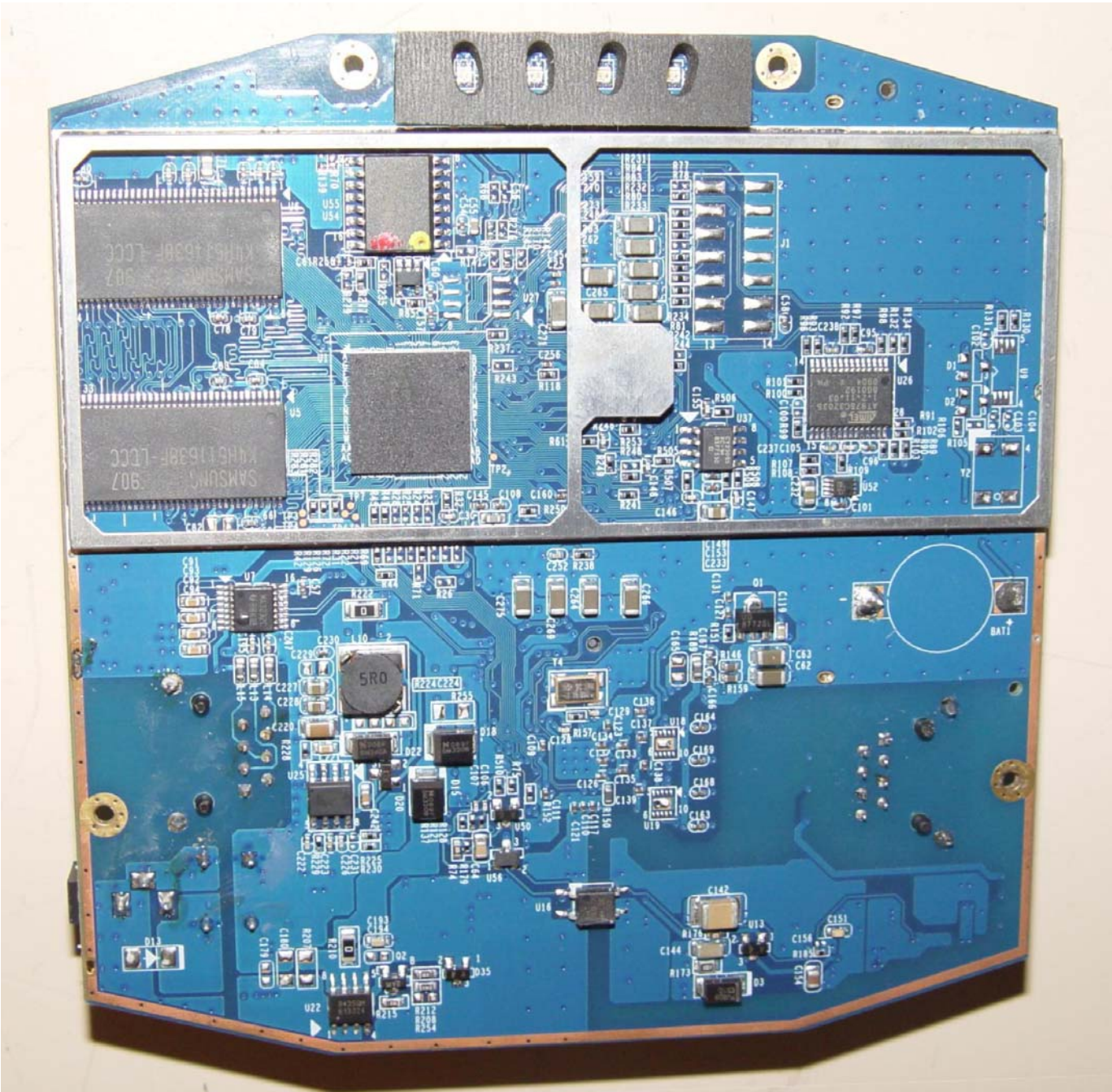
Main Assembly Bottom
