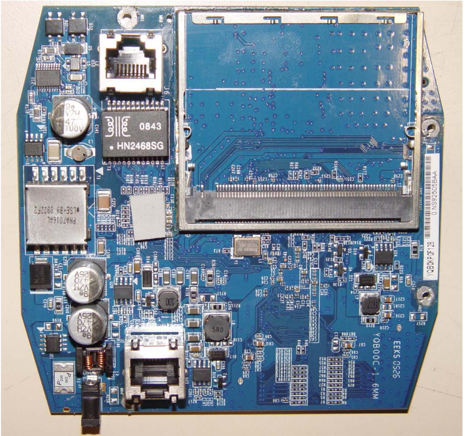
Main Assembly Top
