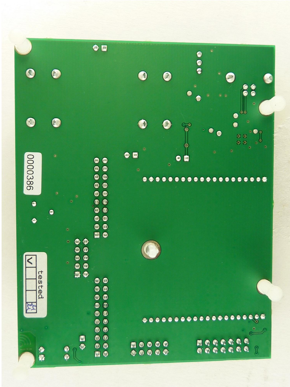
124226_5.JPG: Connector board, bottom view
