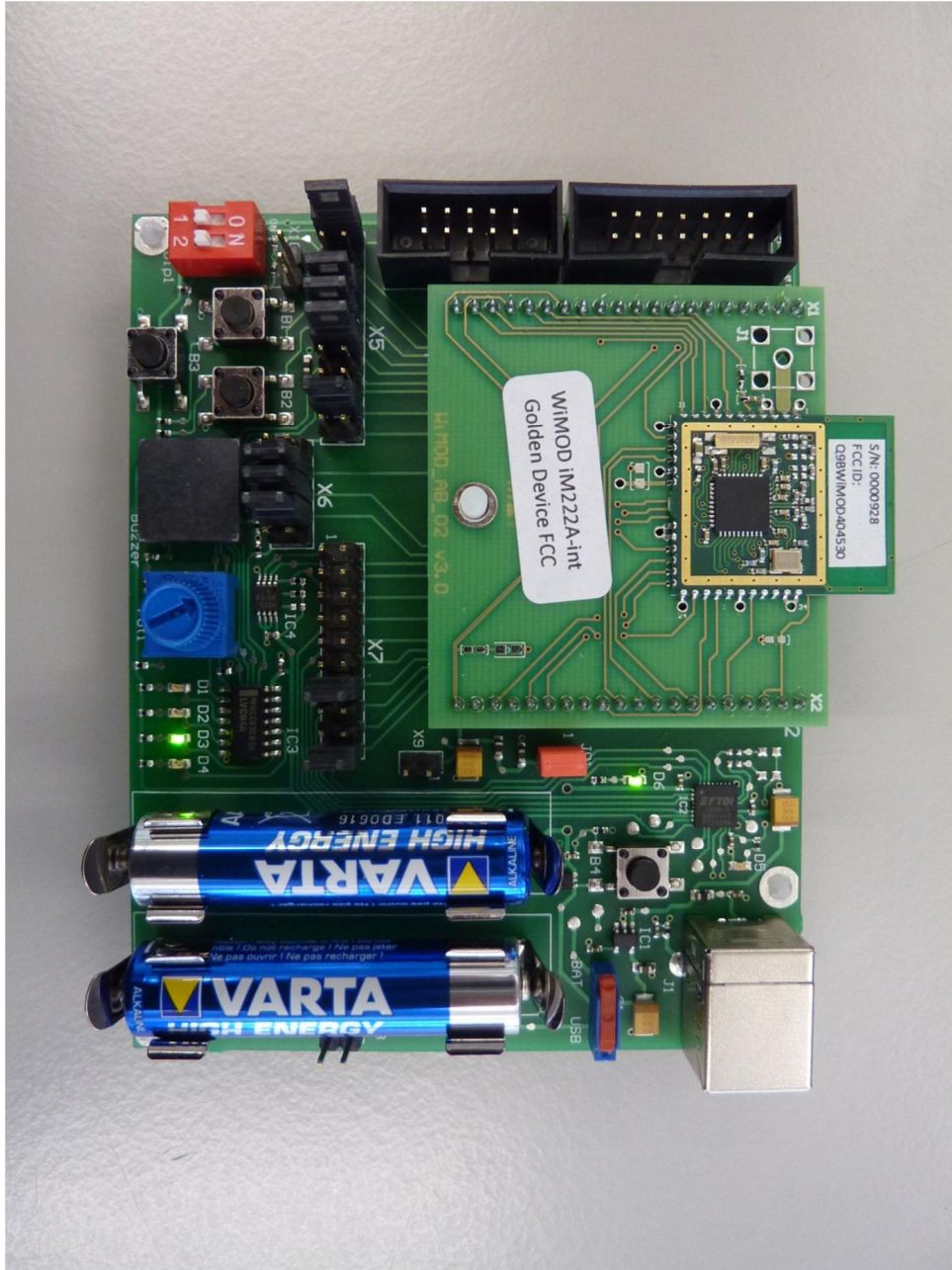
124226_6.JPG: Connector board with mounted carrier board and EUT, top view
