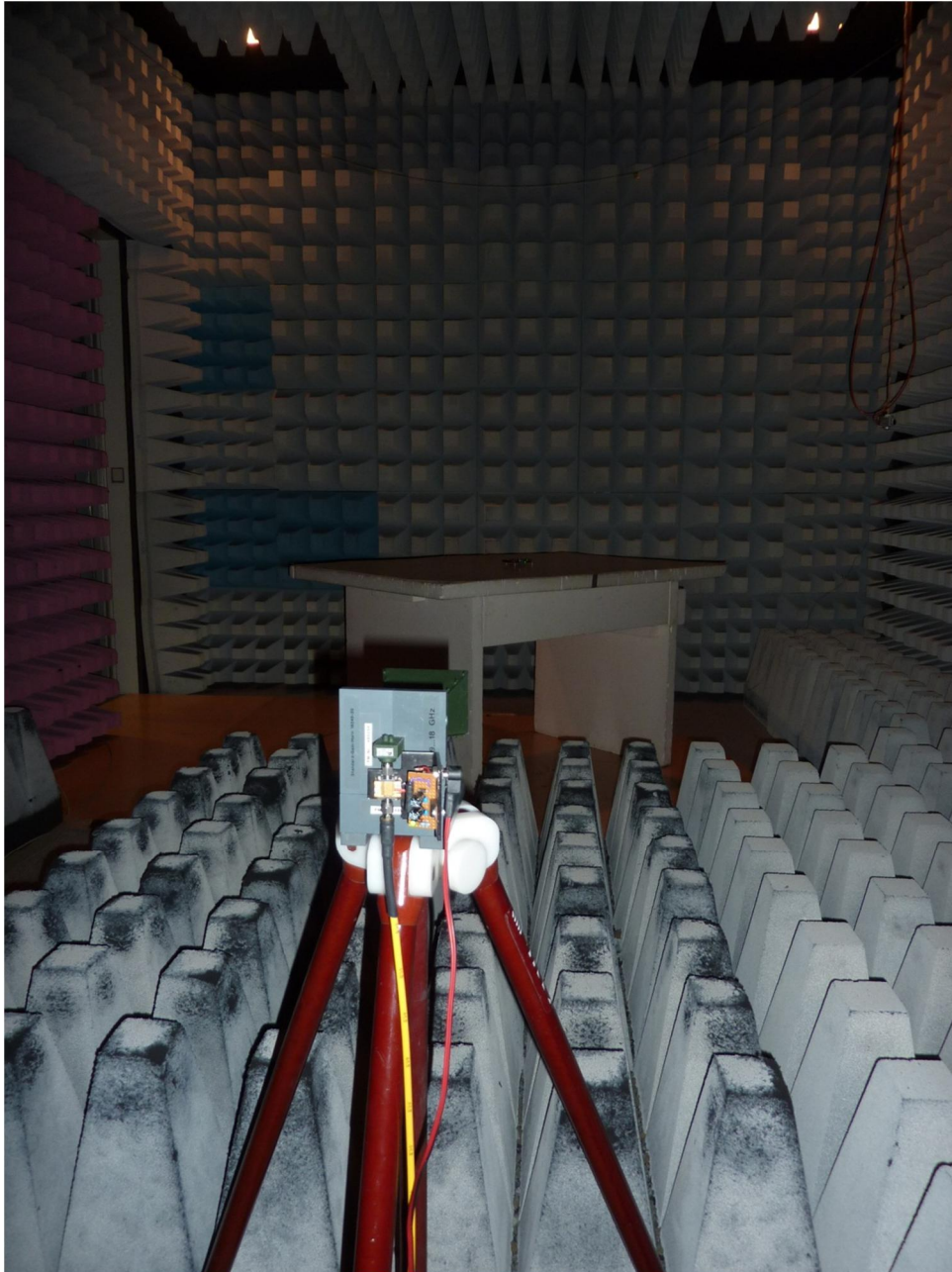
124226_9.JPG: Test setup fully anechoic chamber
