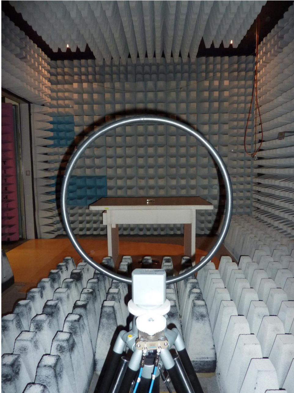
124226_7.JPG: Test setup fully anechoic chamber
