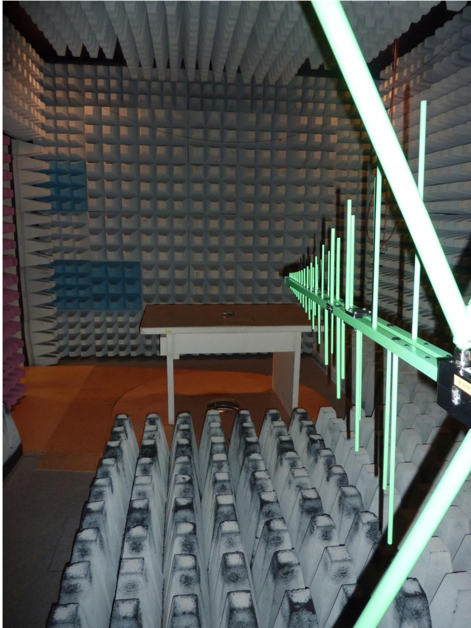
124226_8.JPG: Test setup fully anechoic chamber
