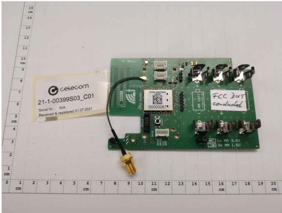
Photograph 1: EUT Top view
