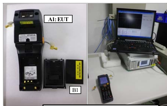
Antenna terminal conducted power measurement
