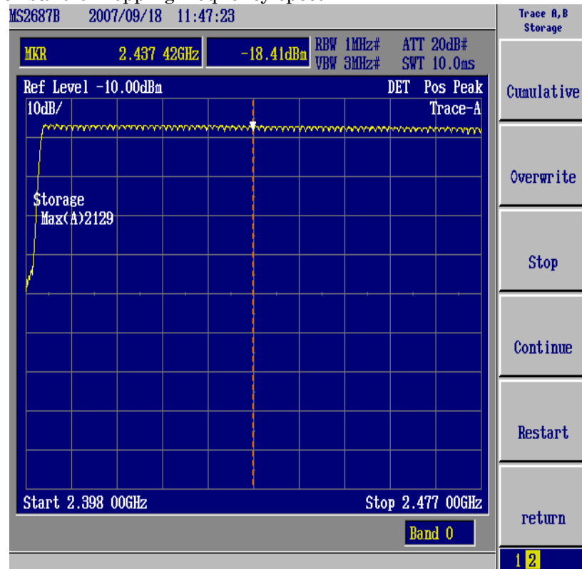
Lower band of hopping frequency spectrum
