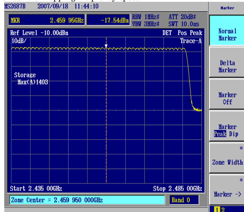
Higher band of hopping frequency spectrum
