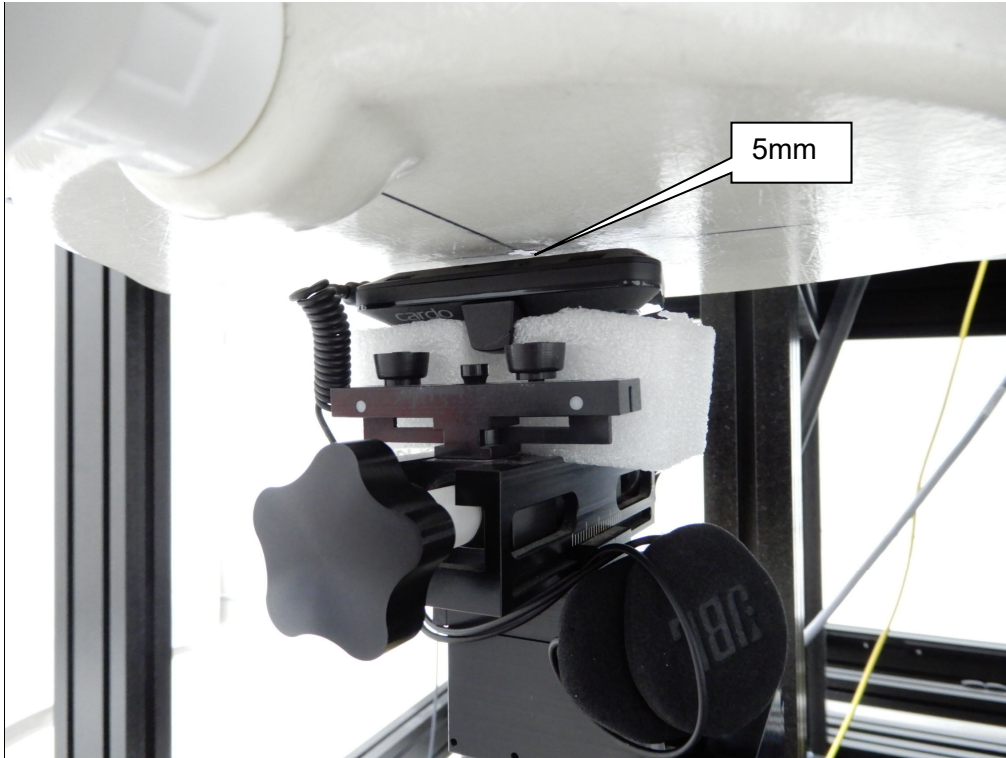
EUT Back_5mm
