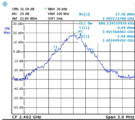
Figure 9. STD, Low
