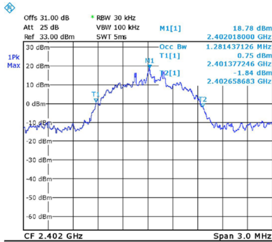
Figure 12. EDR, Low
