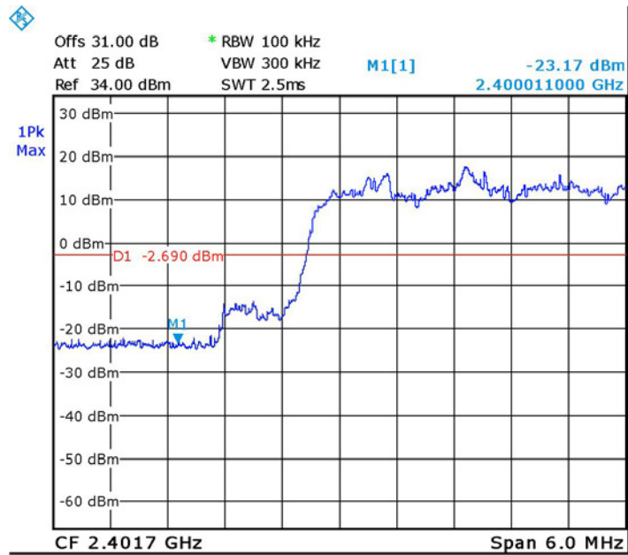
Figure 64 — Hopping - Low EDR Modulation
