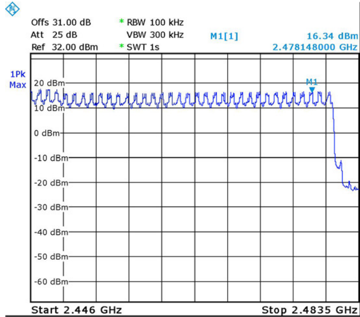
Figure 40. Number of Channels EDR Modulation
