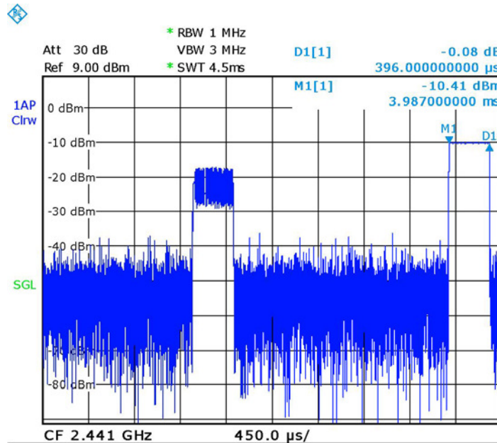
Figure 54 — Number of bursts in 1 sec = 11 standard modulation
