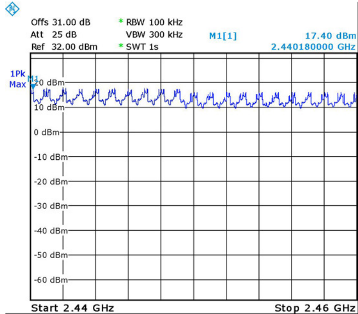
Figure 39. Number of Channels EDR Modulation
