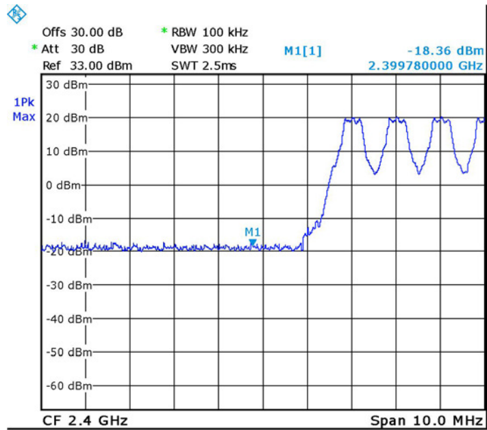
Figure 60 — Hopping - Low Standard Modulation
