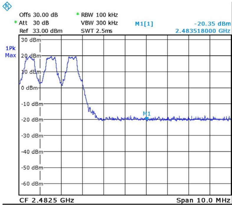
Figure 61 — Hopping - High Standard Modulation
