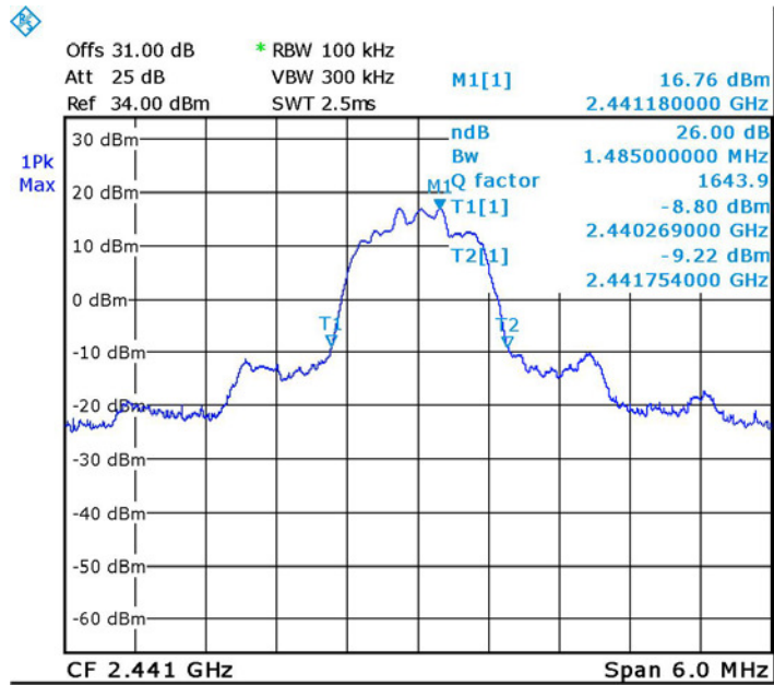
Figure 29. 2441 MHz - Mid EDR Modulation
