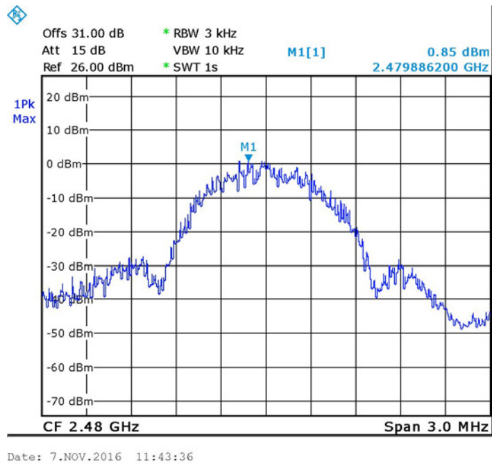
Figure 46 — 2480.0 MHz
