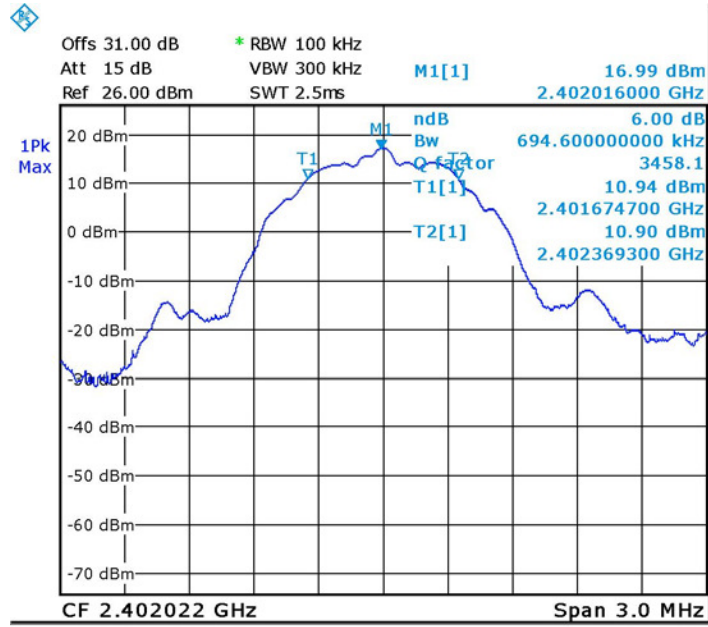
Figure 17. 2402.0 MHz
