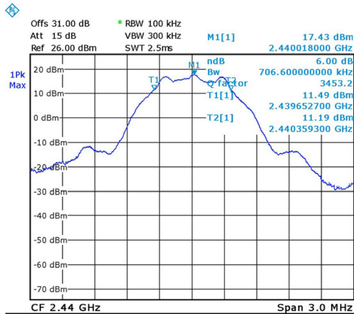
Figure 18. 2440.0 MHz
