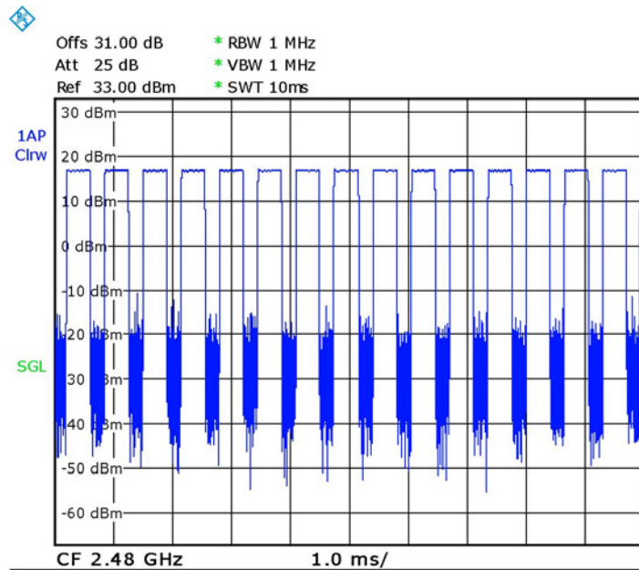
Figure 48. Burst Duration
