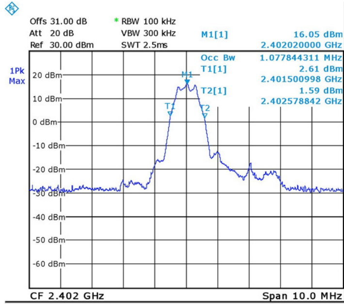
Figure 22. 2402.0 MHz – Occupied Bandwidth
