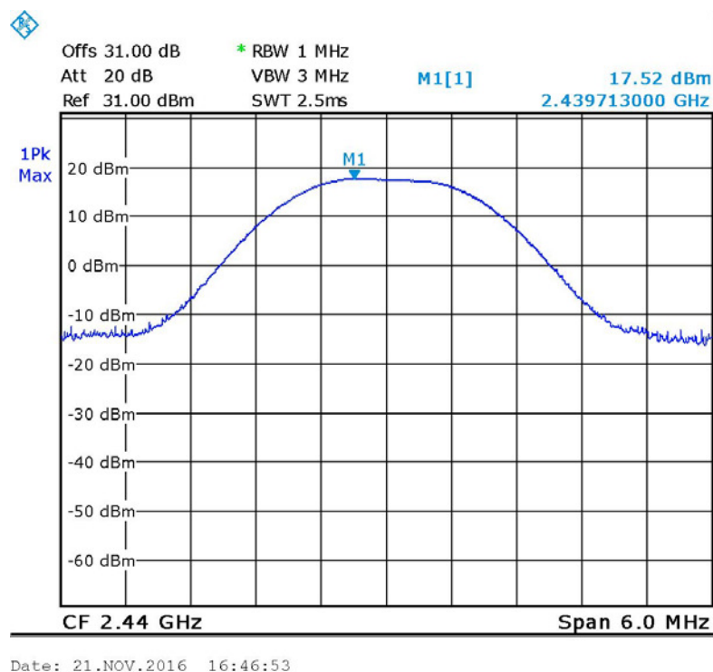
Figure 28 2440.0 MHz
