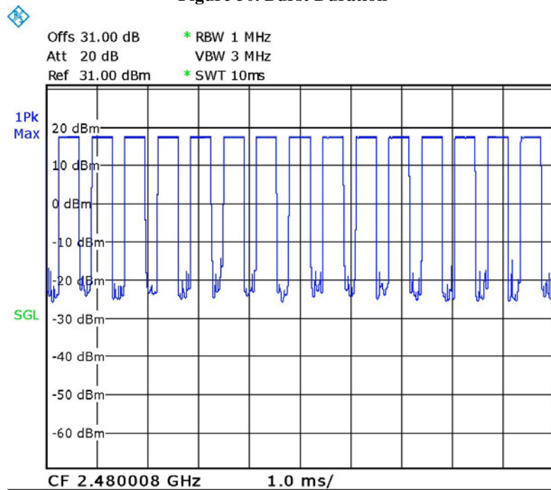
Figure 50. Burst Duration
