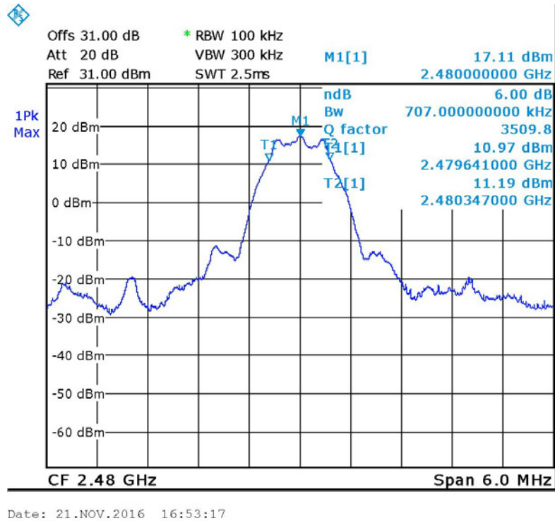
Figure 19. 2480.0 MHz
