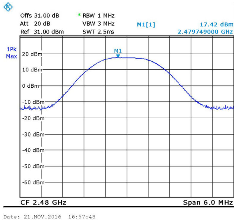
Figure 29 2480.0 MHz
