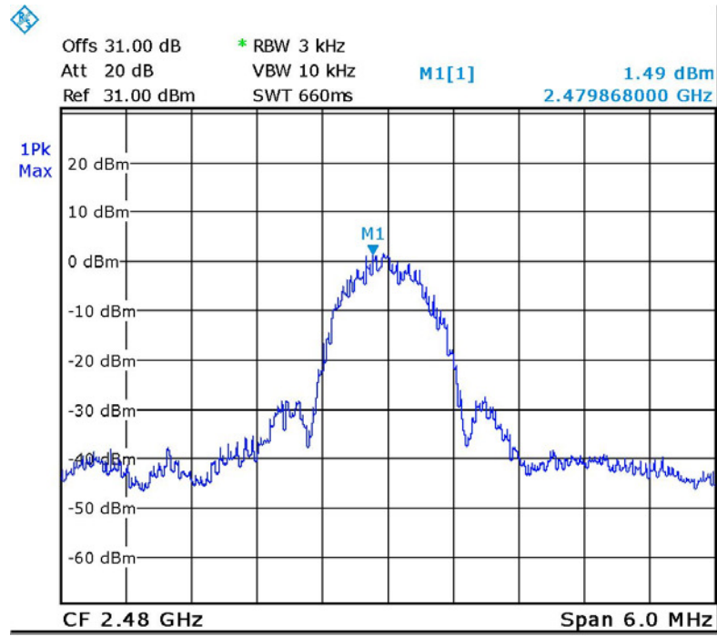
Figure 48 — 2480.0 MHz
