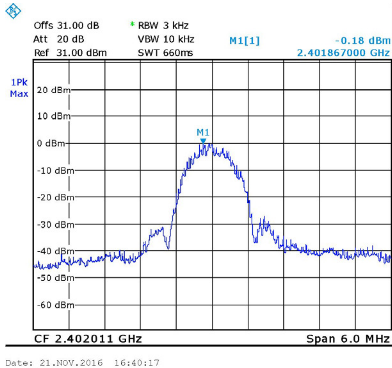
Figure 46 — 2402.0 MHz
