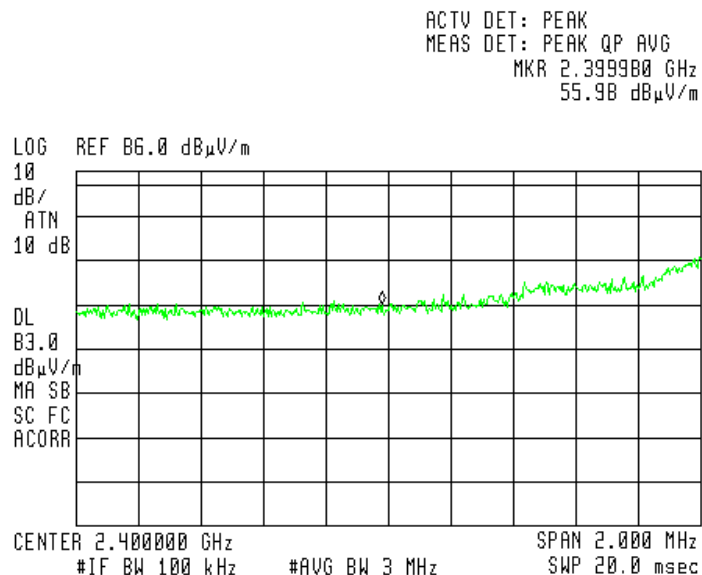
Figure 15 — Q1 Low Channel – Vertical
