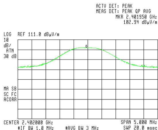
Figure 6 Q1 Low Channel – Vertical
