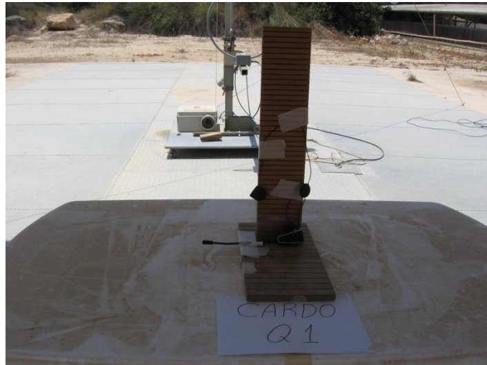
Figure 2 Q1 Radiated Emission 9kHz -30 MHz
