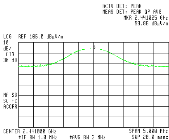
Figure 8 Q1 Mid Channel – Vertical
