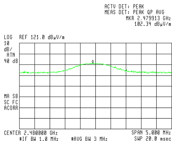
Figure 10 Q1 High Channel – Vertical
