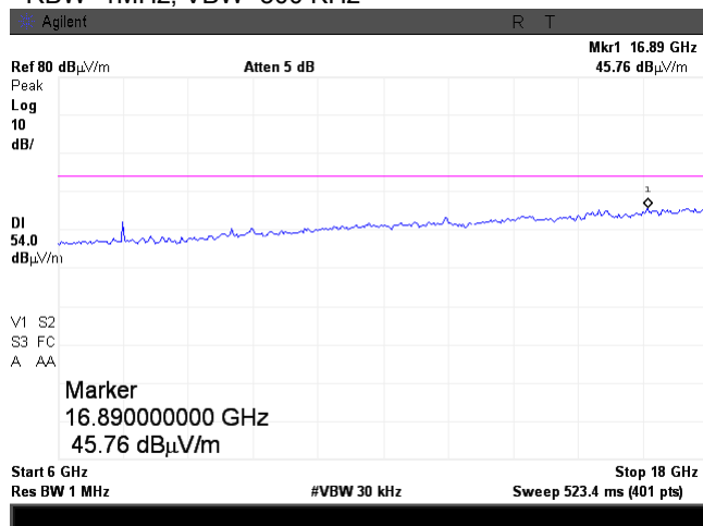
Plot 7.9.28 Radiated emission measurements from 6.0 to 18.0GHz at the mid carrier frequency
