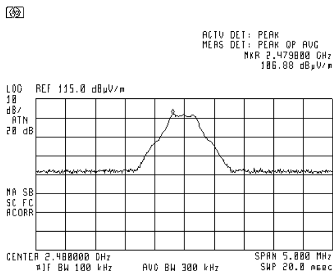
Plot 7.7.2 The highest emission level within the assigned band at high carrier frequency
