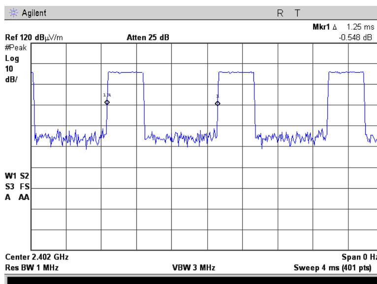
Plot 7.9.43 Transmission pulse period
