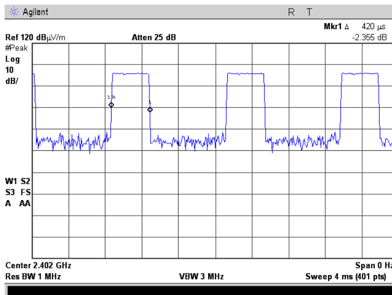
Plot 7.6.7 Transmitter duty cycle, pulse duration
