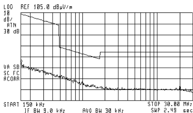
Plot 7.9.9 Radiated emission measurements from 0.15 to 30 MHz at the high carrier frequency
