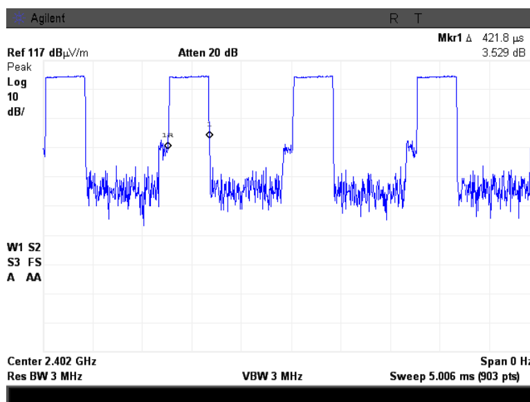
Plot 7.10.52 Transmission pulse duration
