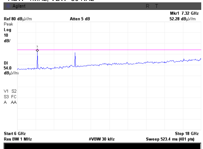
Plot 7.10.29 Radiated emission measurements from 6.0 to 18.0 GHz at the high carrier frequency
