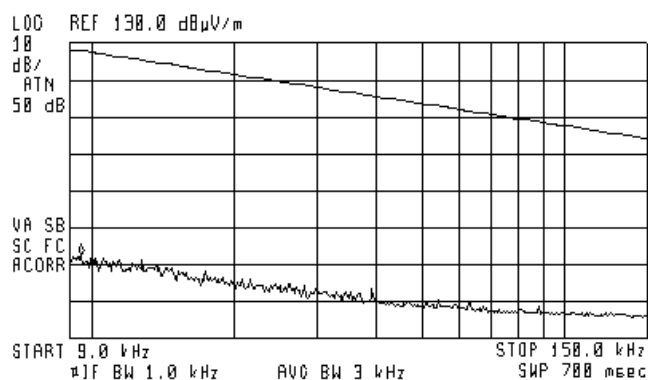
Plot 7.9.5 Radiated emission measurements from 9 to 150 kHz at the mid carrier frequency
