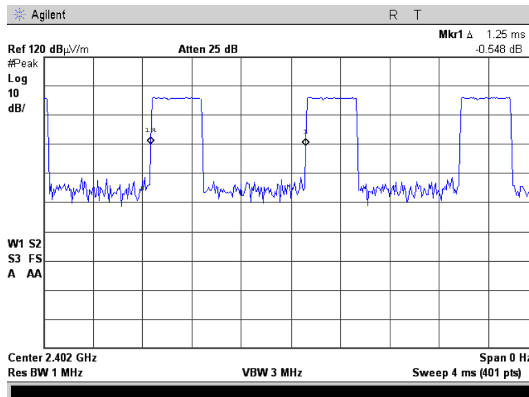
Plot 7.5.8 Transmitter duty cycle, pulse period
