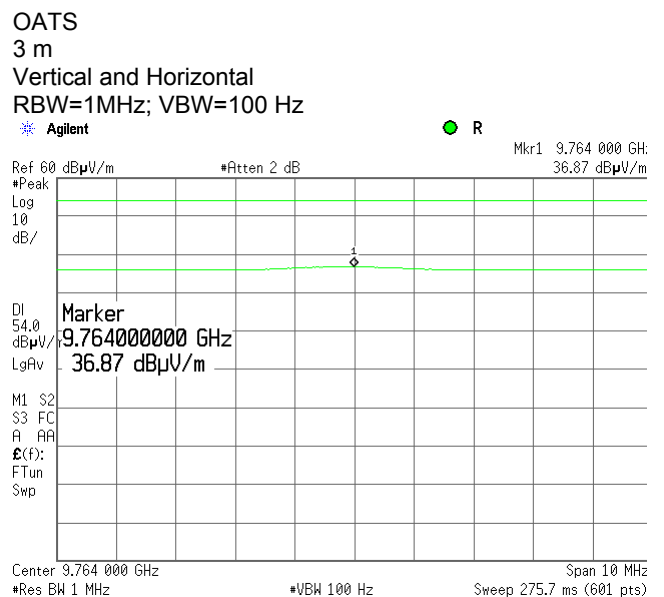
Plot 7.9.40 Radiated emission measurements at the fourth harmonic of mid carrier frequency
