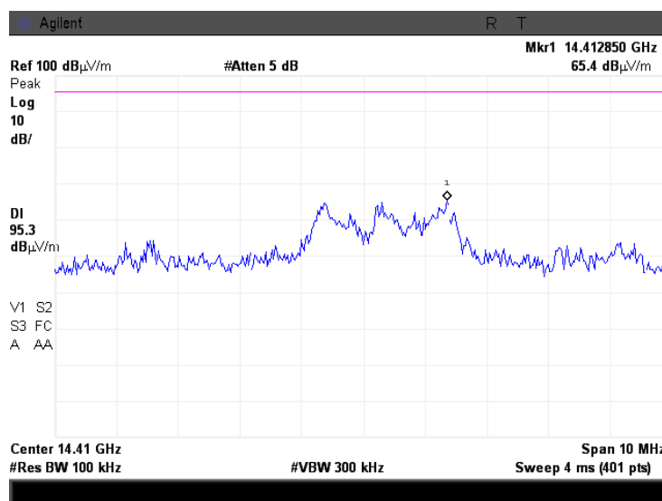
Plot 7.10.46 Radiated emission measurements at the sixth harmonic of mid carrier frequency
