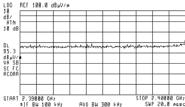
Plot 7.8.4 The highest band edge emission at low carrier frequency with hopping function disabled
