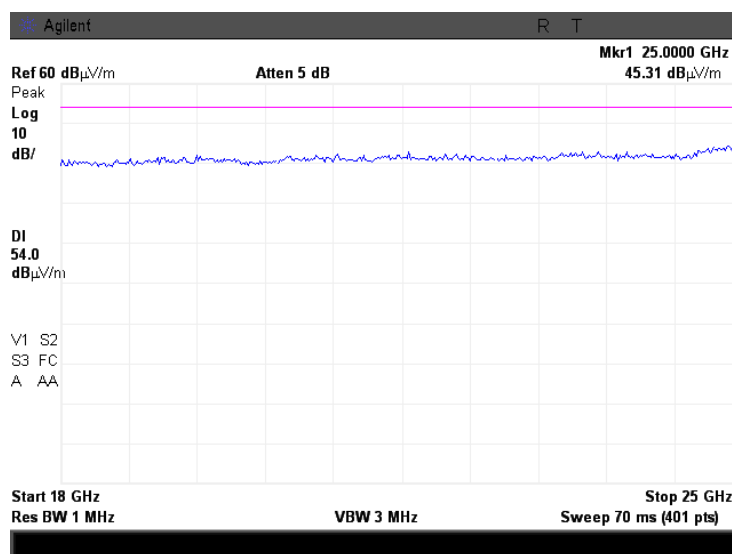
Plot 7.9.32 Radiated emission measurements from 18.0 to 25.0 GHz at the high carrier frequency
