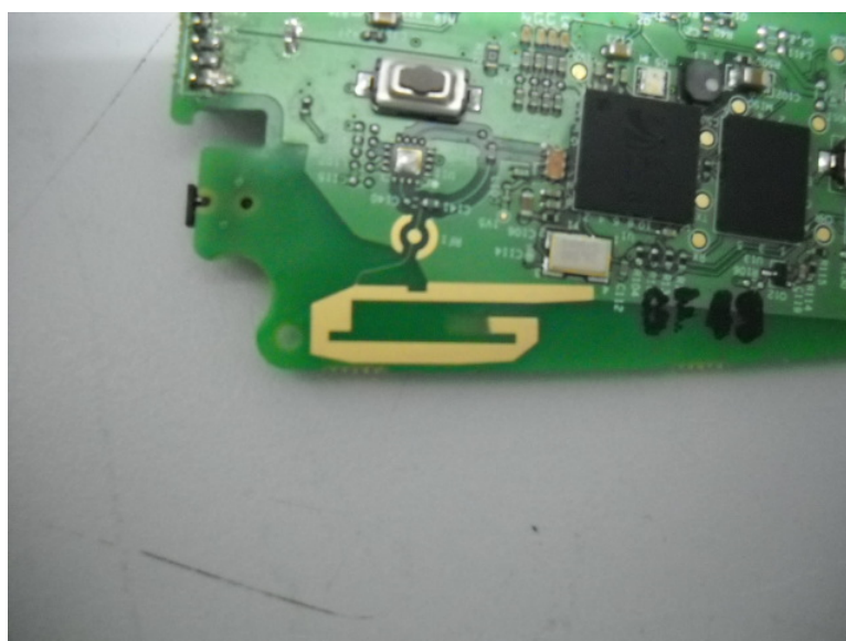
Photograph 7.11.2 Antenna assembly of “scala rider Q1”
