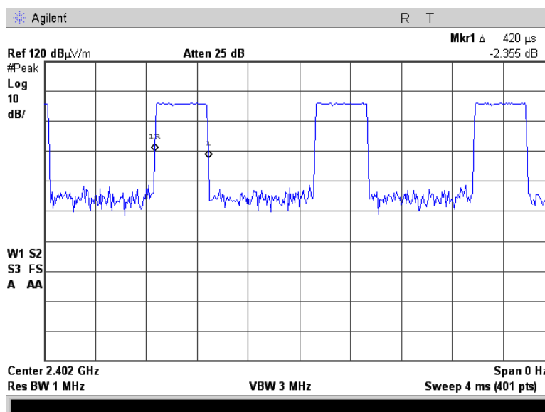
Plot 7.9.42 Transmission pulse duration
