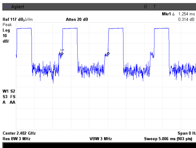
Plot 7.10.53 Transmission pulse period
