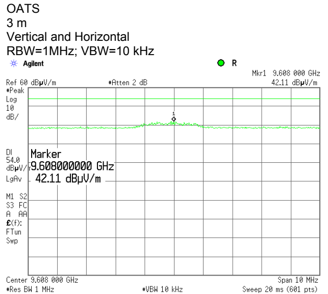
Plot 7.9.39 Radiated emission measurements at the fourth harmonic of low carrier frequency
