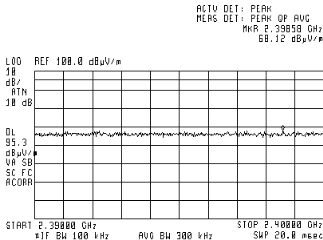
Plot 7.8.7 The highest band edge emission at low carrier frequency with hopping function enabled
