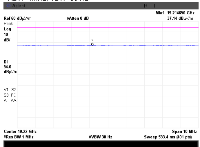
Plot 7.10.51 Radiated emission measurements at the eighth harmonic of mid carrier frequency
