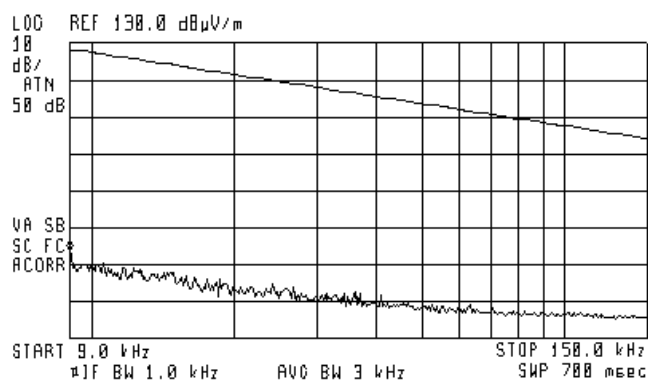
Plot 7.10.5 Radiated emission measurements from 9 to 150 kHz at the mid carrier frequency
