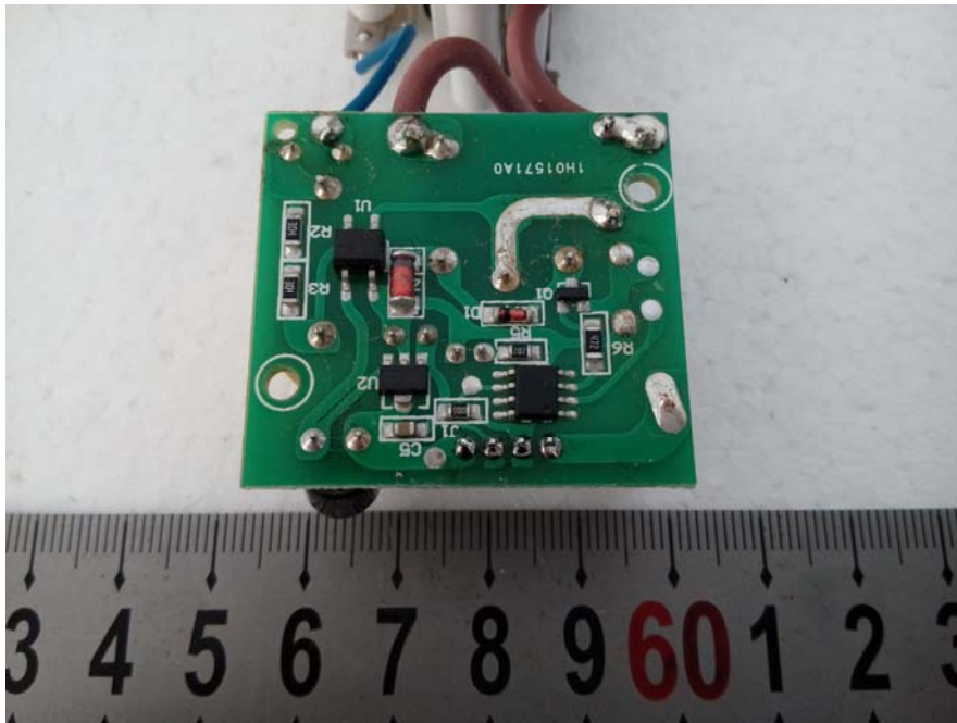
EUT –Main board Bottom View(BHC9938U and C-9938-Receiver)
