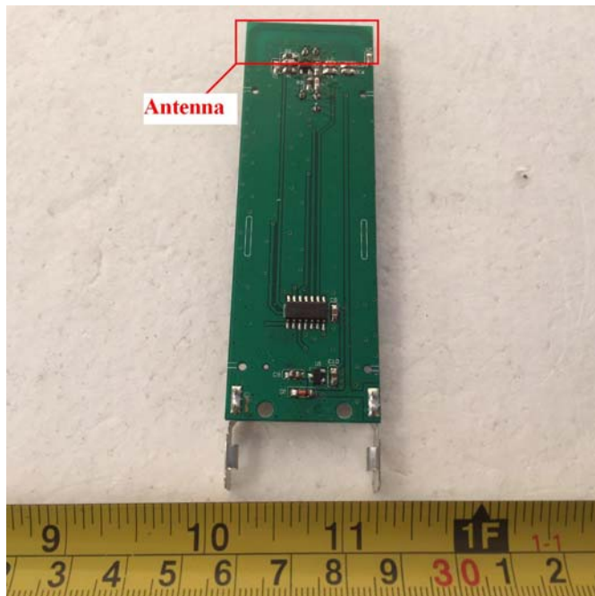
EUT - Main Board & Antenna View
