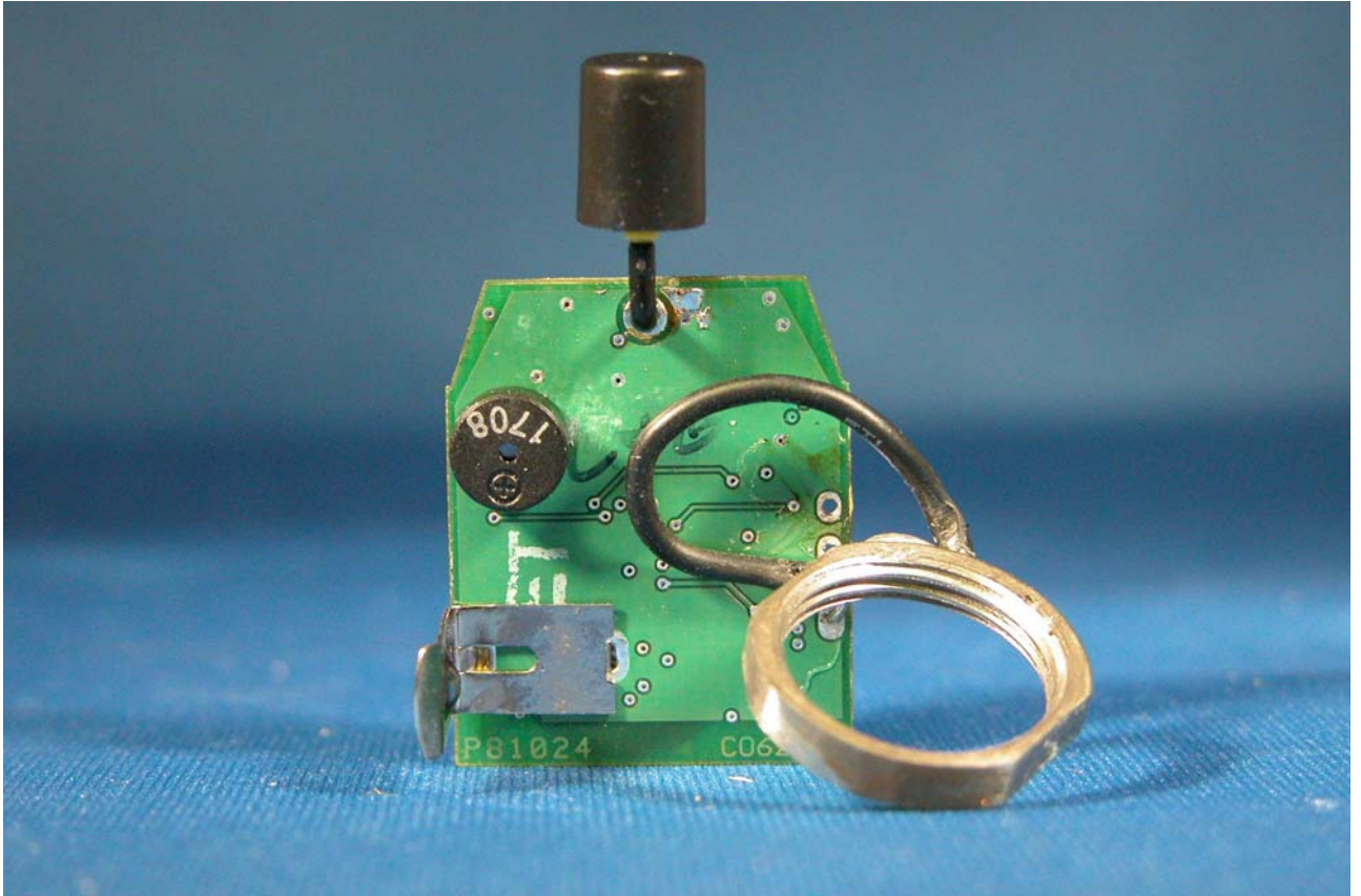
Receiver/Collar internal rear PCB
