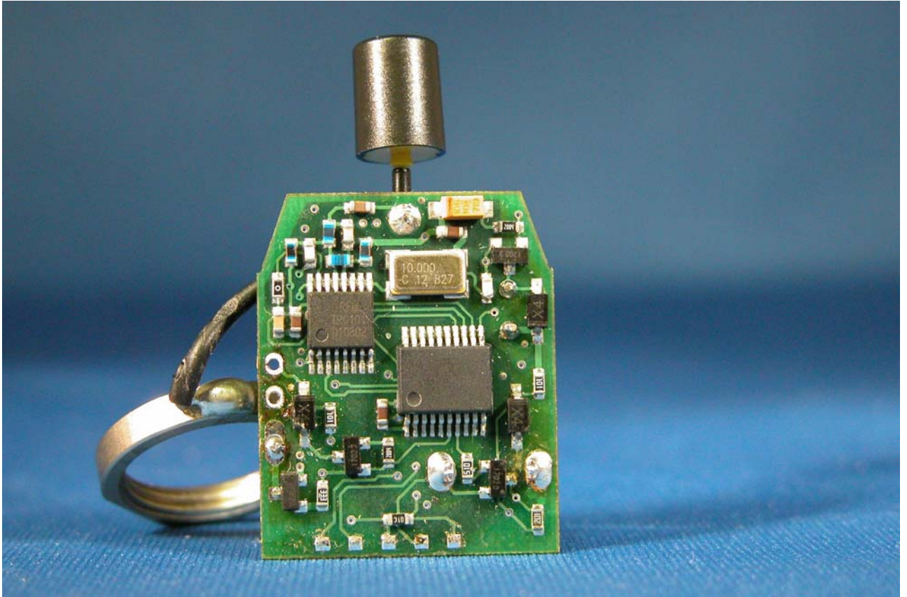
Receiver/Collar internal front PCB
