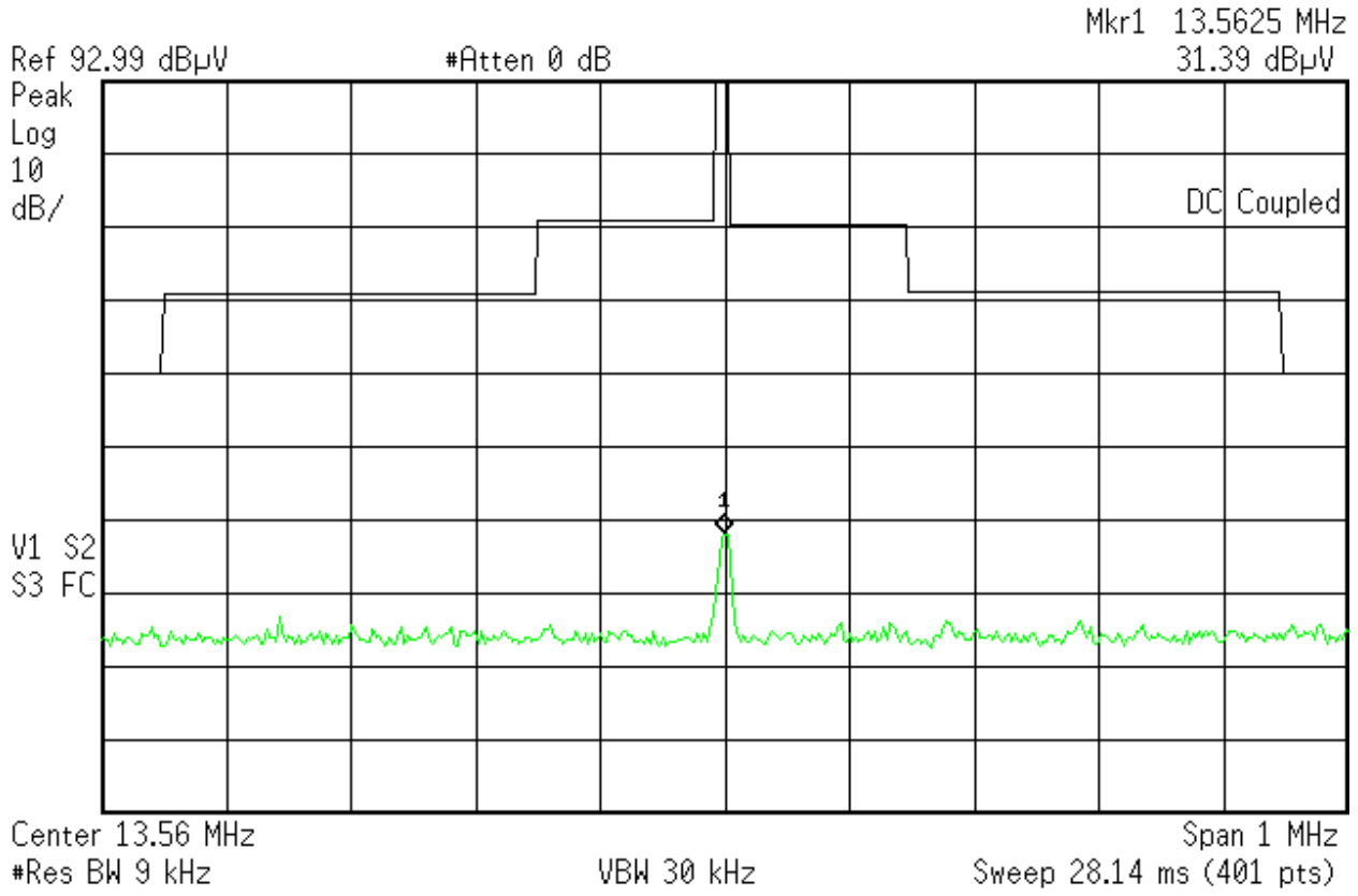
Spectrum Mask Limits - 90 Degree Polarization
