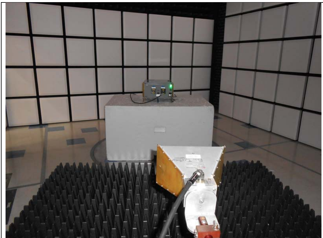
RF Radiated #2_above 1 GHz NEMA Enclosure
