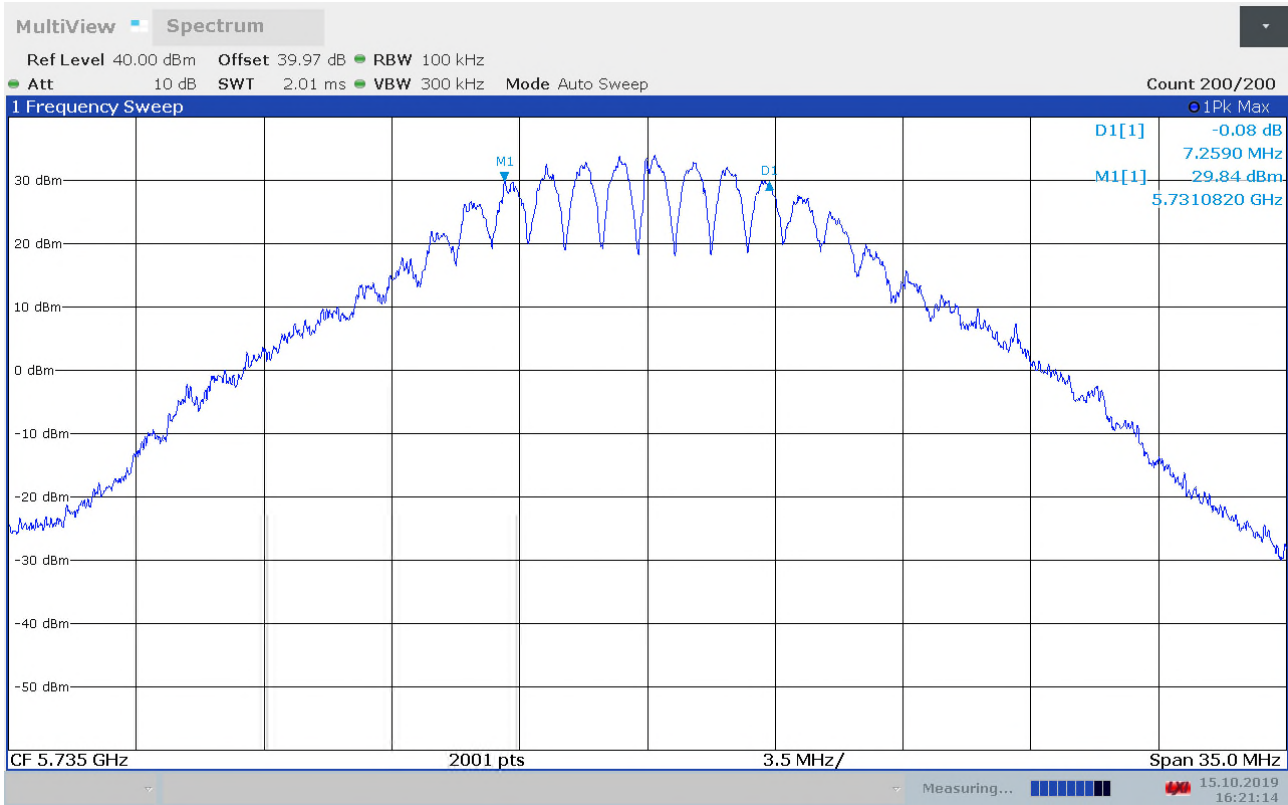
DTS Bandwidth, 5735 MHz
