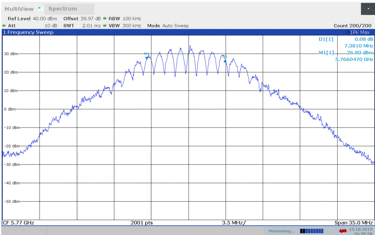
DTS Bandwidth, 5770 MHz
