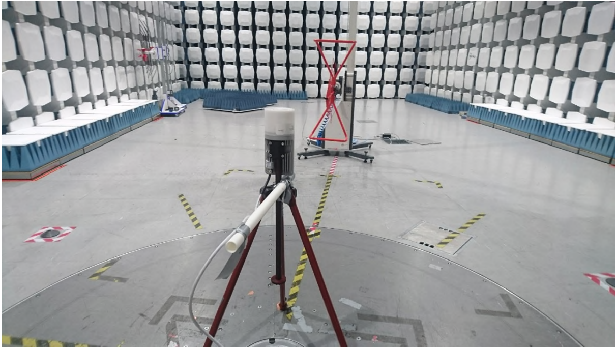
Radiated Emissions, 30 - 1000 MHz
