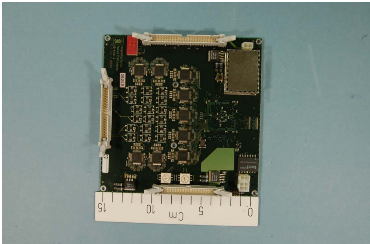
Pre-processor board front view- interrogator
