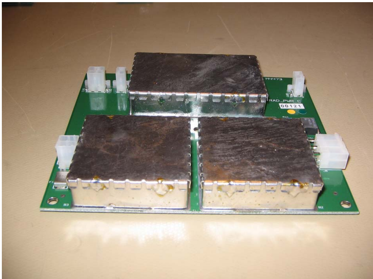
Power board front view - interrogator
