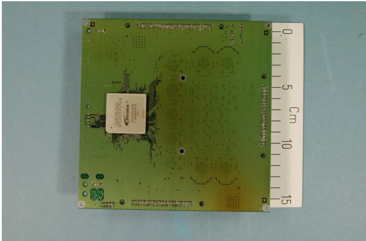
Pre-processor board rear view- interrogator
