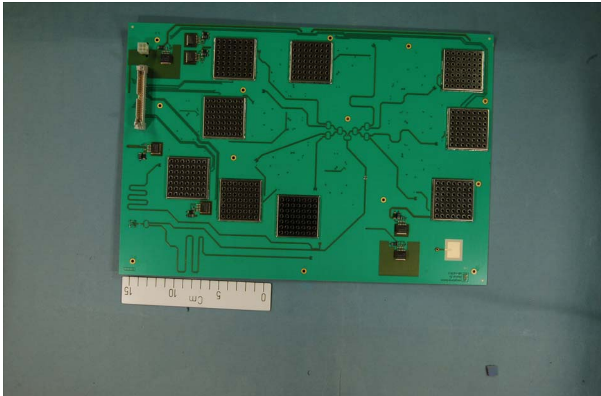
Rear side of patch antenna – interrogator
