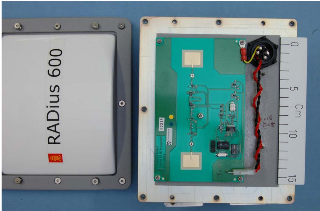
High gain transponder 600 - Front View of the PCB
