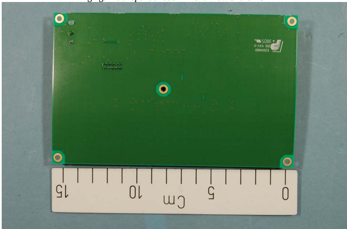
High gain transponder 600 - Rear View of the PCB
