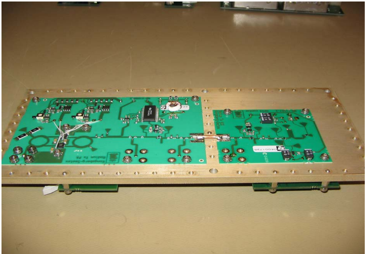
TX VCO and TX PA boards - interrogator
