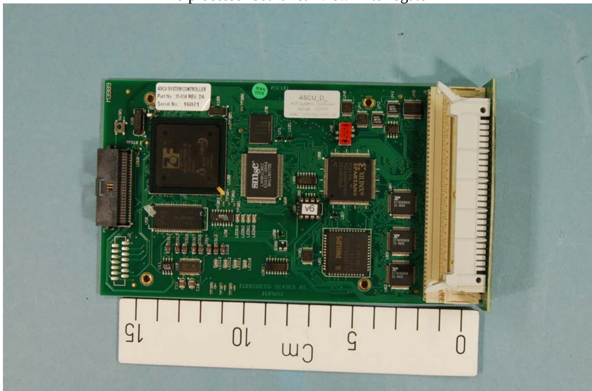
ASCU system controller front view- interrogator
