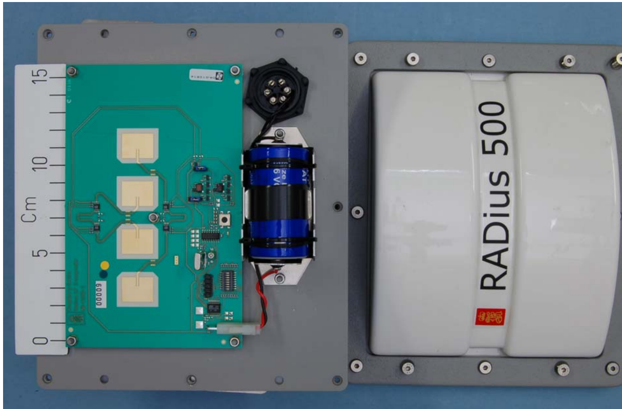
Low power transponder 500 – Front View of the PCB
