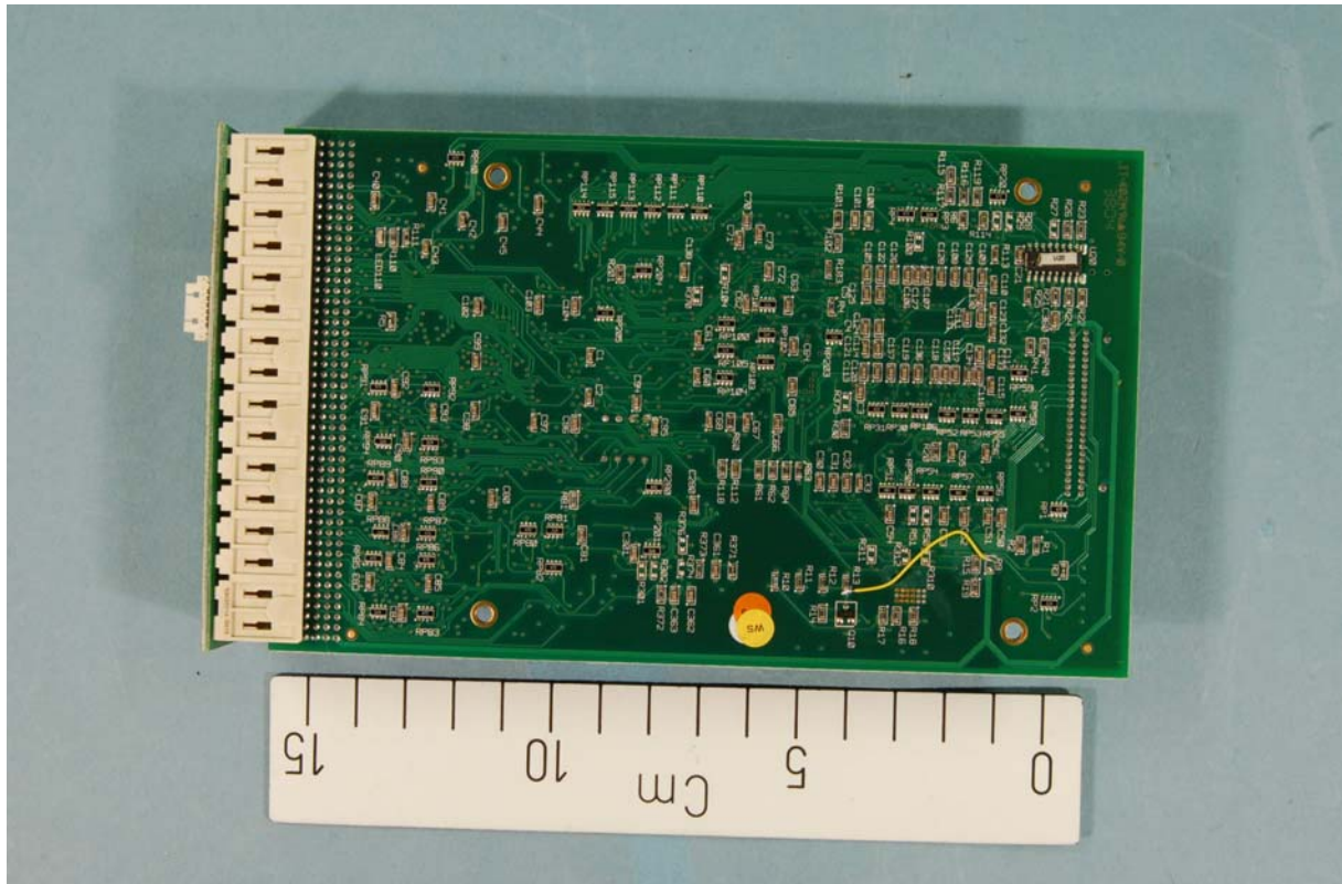
ASCU system controller rear view- interrogator
