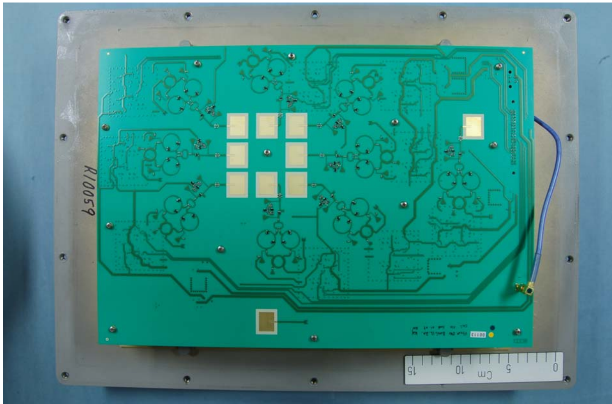
View of the interrogator patch antenna
