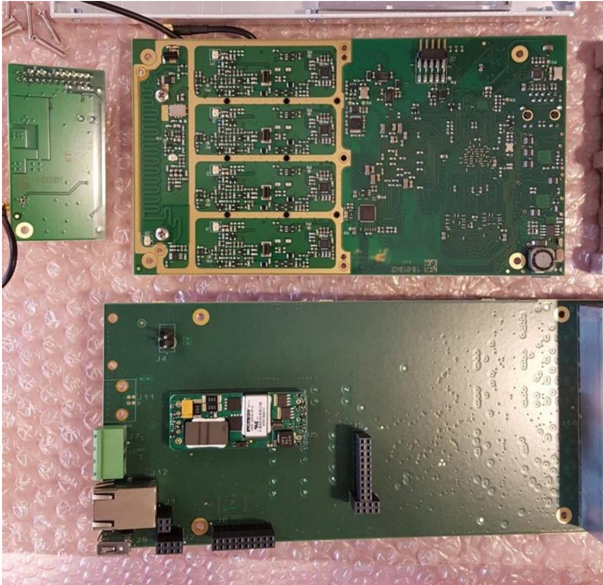
Figur 4 AIS 300 Circuit boards rear – without shields
