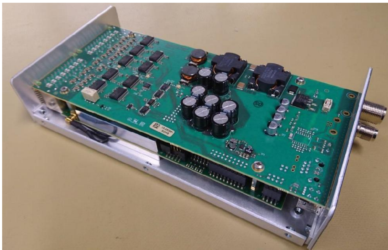
Figure 1 AIS 300 Interface board mounted onto AIS main board
