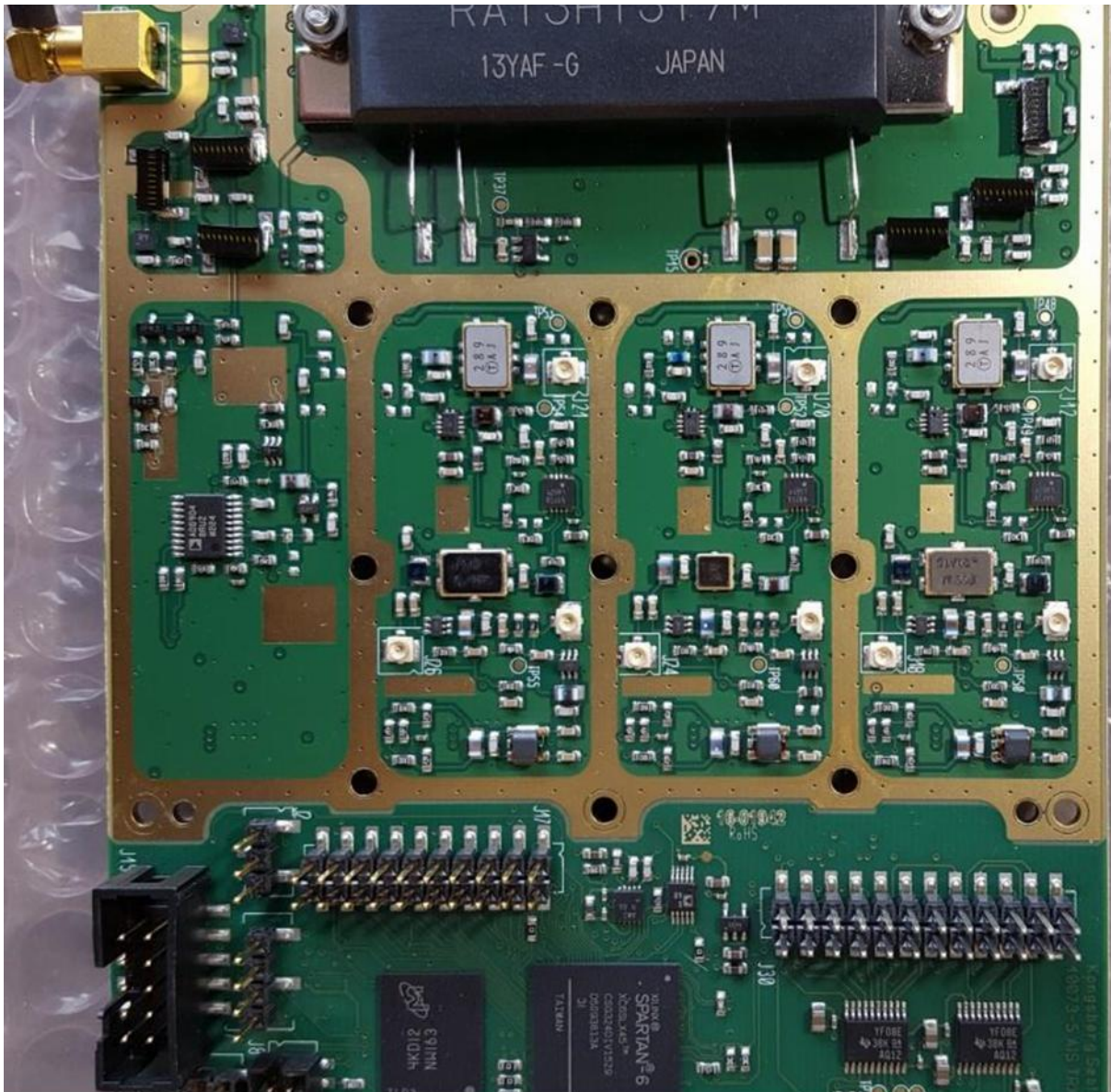
Figur 5 AIS 300 radio without shield - details
