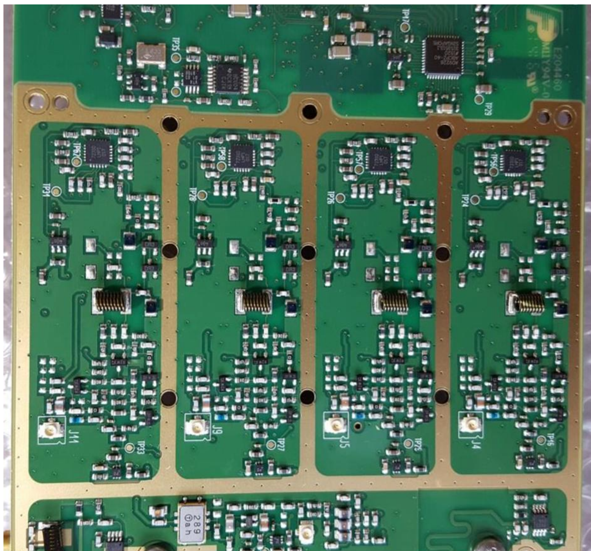
Figur 6 AIS 300 radio without shield - rear
