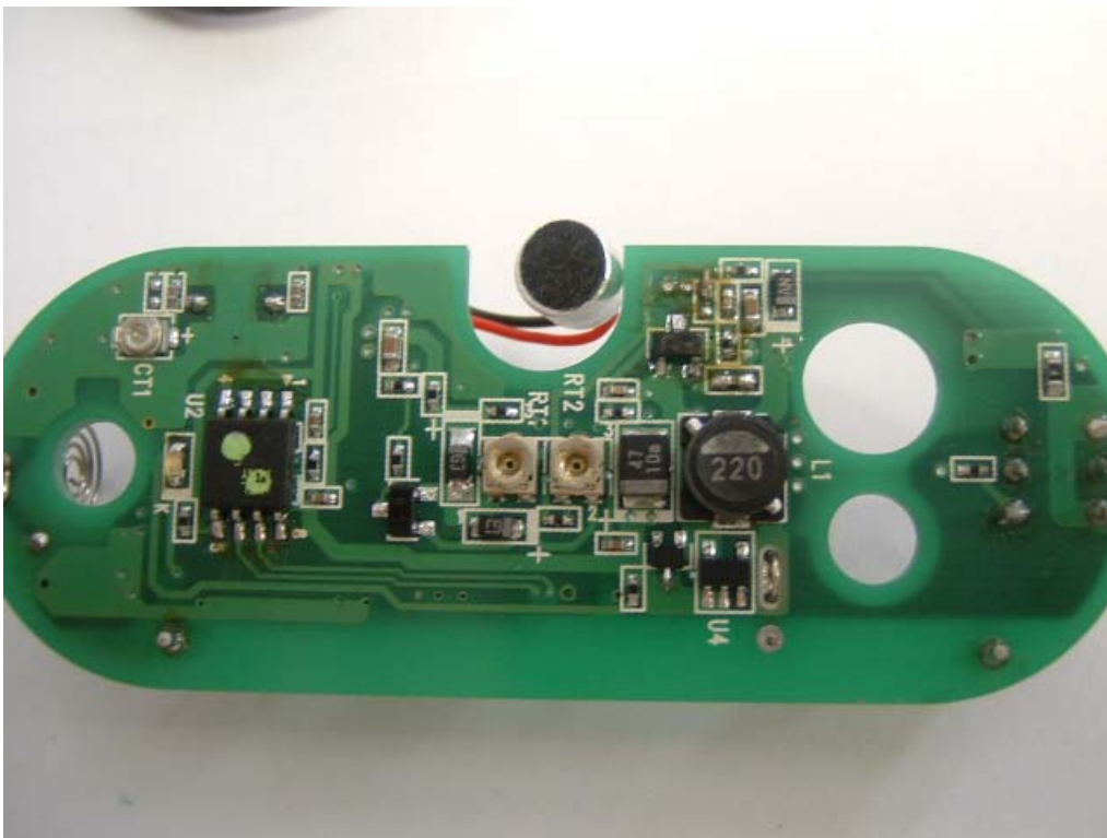
PWB Back
