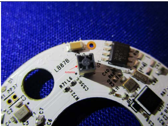
Antenna View
