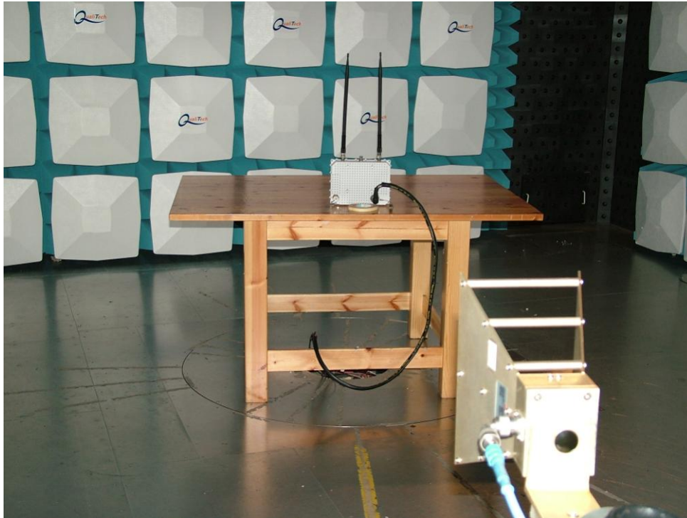
Photograph 3: Radiated Measurements
