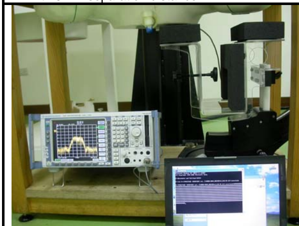
Test Setup
