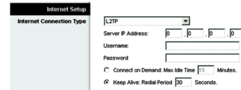
Figure 5-7: L2TP
