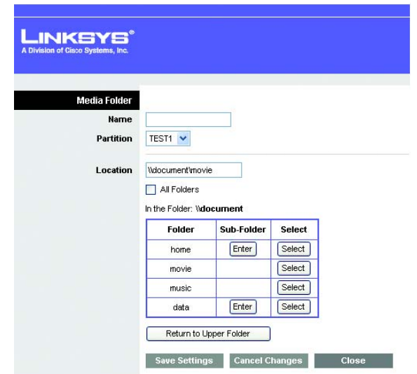
Figure 5-29: Media Folder
