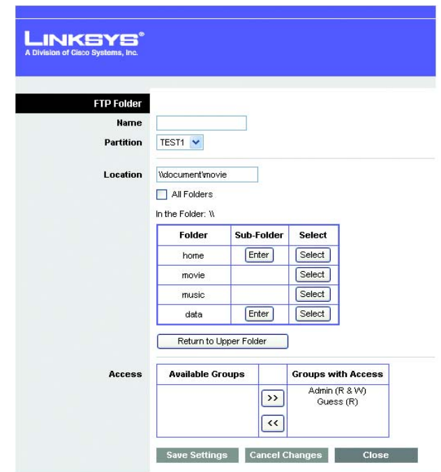
Figure 5-31: FTP Folder
