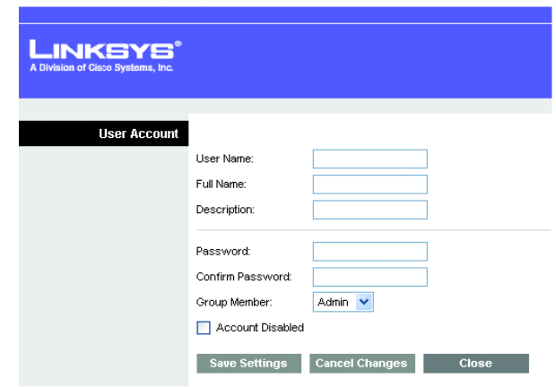
Figure 5-33: User Account
