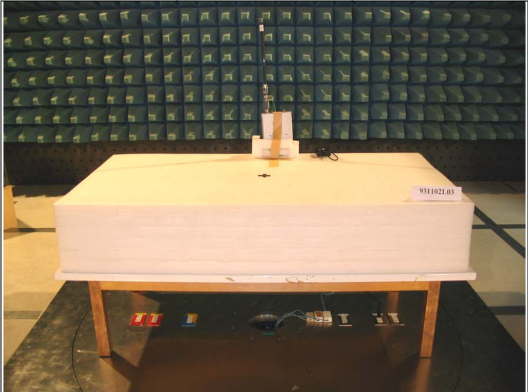
(Omnidirectional Antenna)
