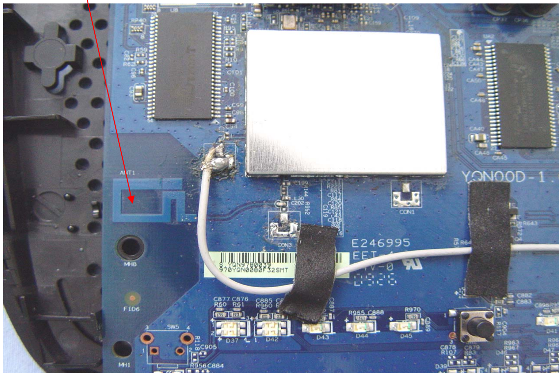
PCB Antenna
