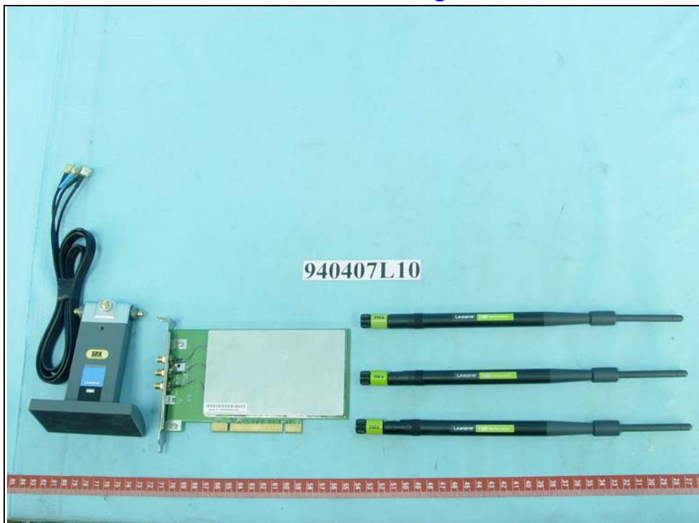
Antenna with 7dBi gain
