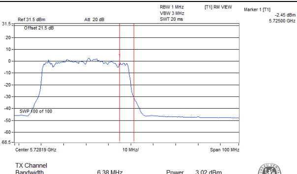
802.11ac (VHT40)_Chain 0 / CH142 (U-NII-3 Band)
