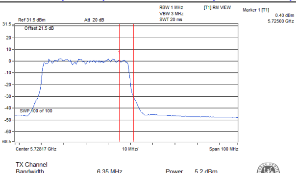
802.11ac (VHT40)_Chain 1 / CH142 (U-NII-3 Band)
