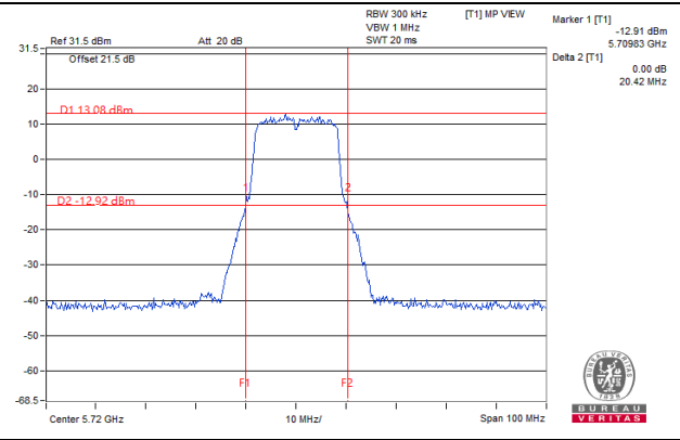
802.11ax (HE20)_Chain 0/ CH144 (U-NII-2C Band)
