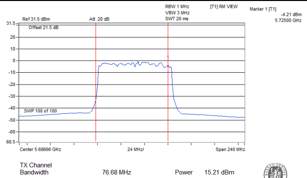
802.11ac (VHT80)_Chain 0 / CH138 (U-NII-2C Band)
