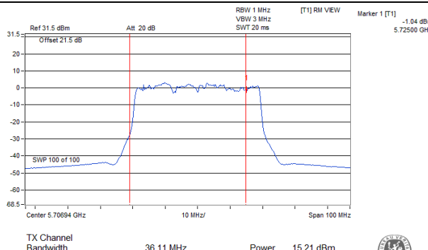
802.11ac (VHT40)_Chain 0 / CH142 (U-NII-2C Band)
