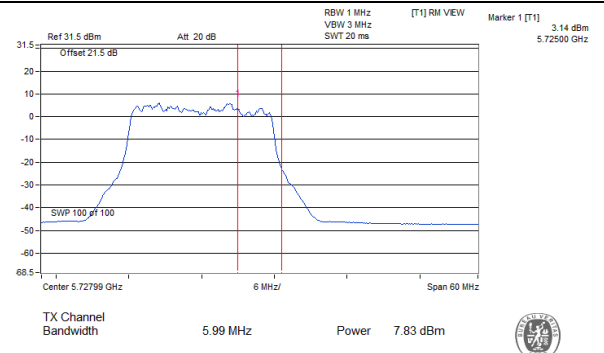
802.11ac (VHT20)_Chain 1 / CH144 (U-NII-3 Band)
