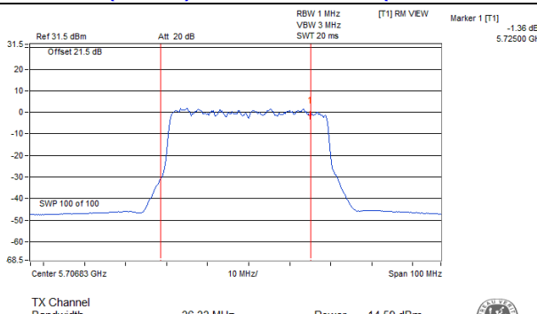
802.11ac (VHT40)_Chain 1 / CH142 (U-NII-2C Band)
