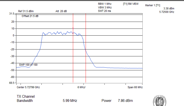
802.11ax (HE20)_Chain 1 / CH144 (U-NII-3 Band)
