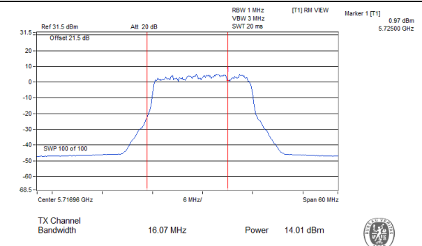
802.11ac (VHT20)_Chain 1 / CH144 (U-NII-2C Band)
