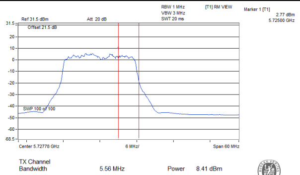
802.11ac (VHT20)_Chain 0 / CH144 (U-NII-3 Band)
