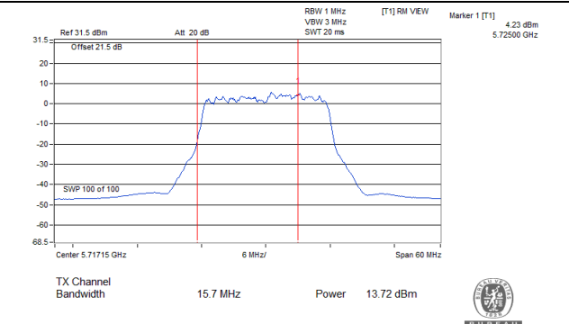
802.11ax (HE20)_Chain 0 / CH144 (U-NII-2C Band)
