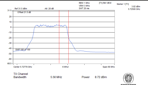
802.11ax (HE20)_Chain 0 / CH144 (U-NII-3 Band)
