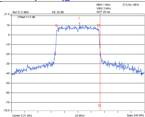
802.11ac(VHT80)_Chain0 / CH42
