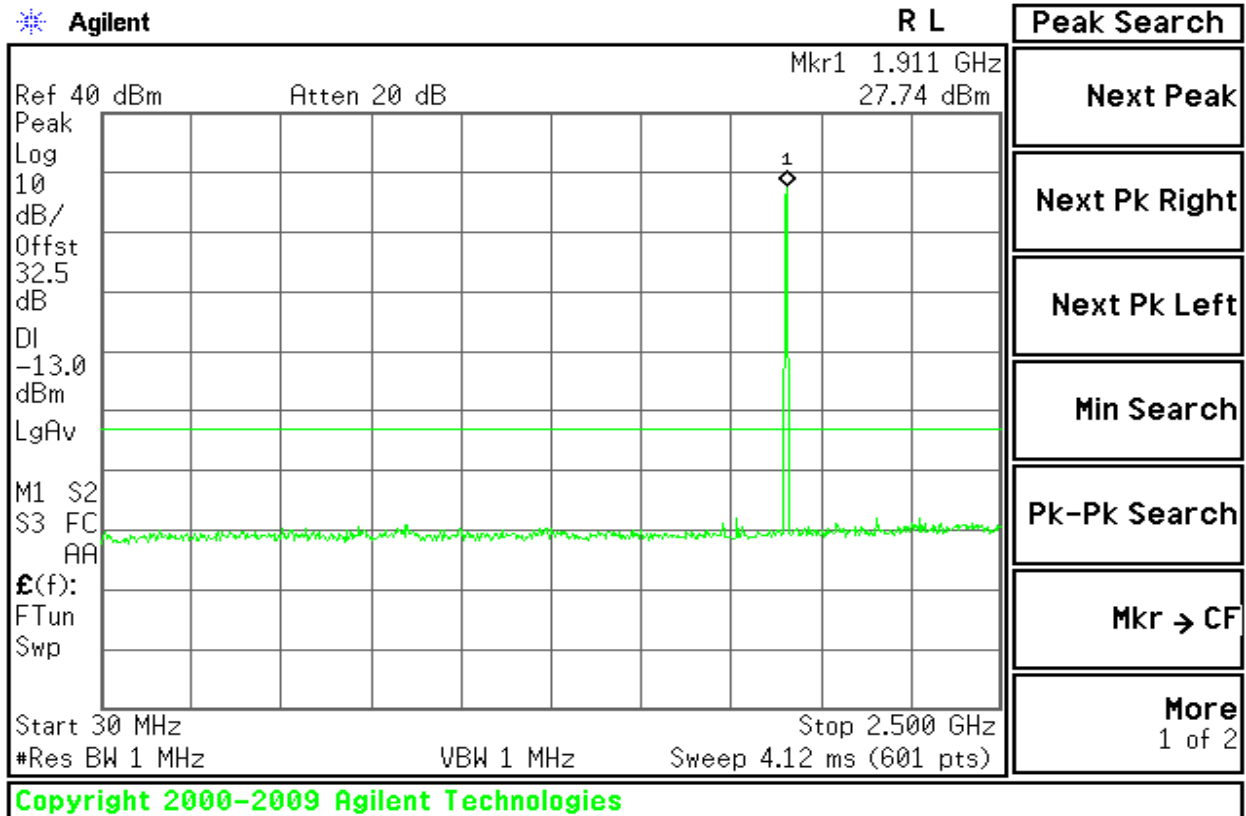
Figure 8-12: Out of Band emission at antenna terminals – GSM CH High
