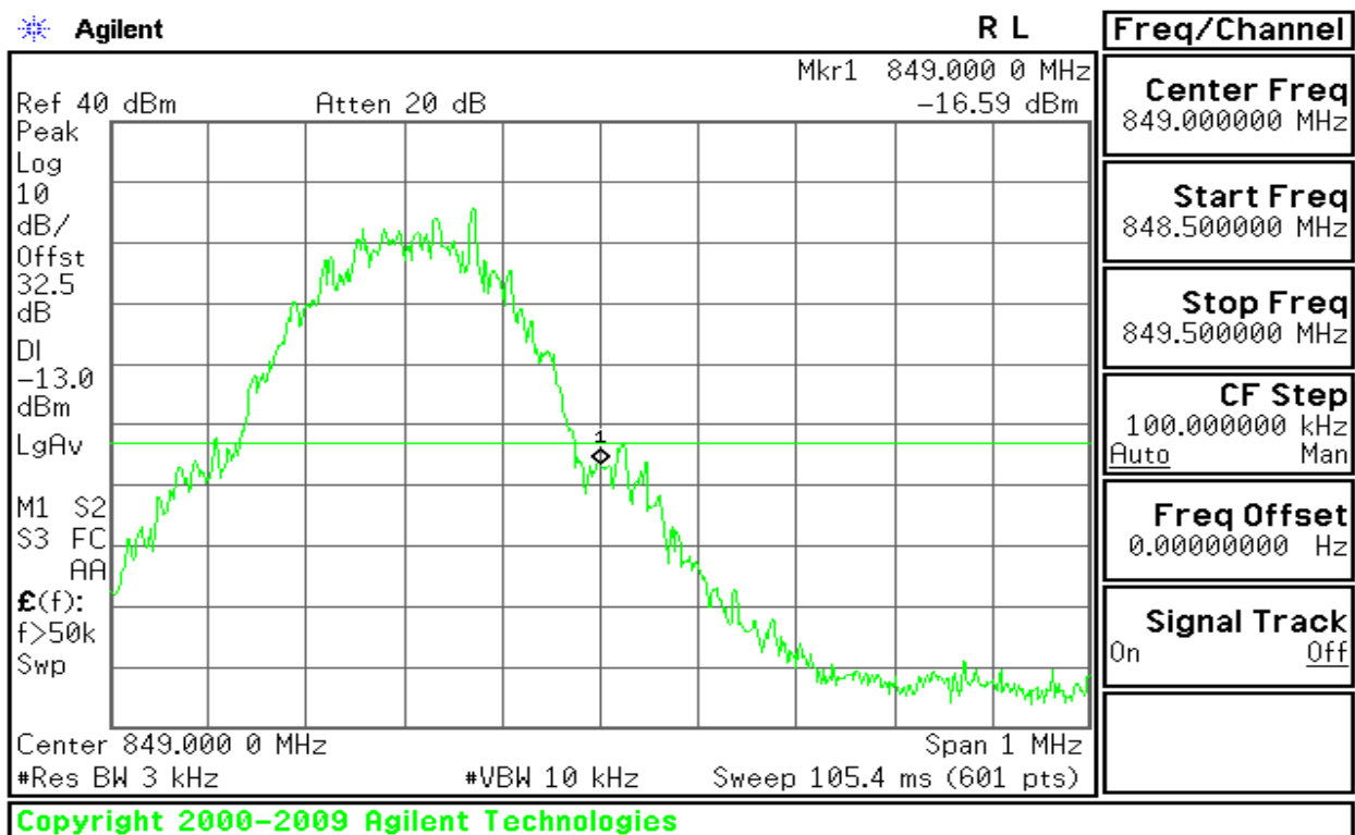
Figure 9-4: Band Edge emissions – GPRS CH High
