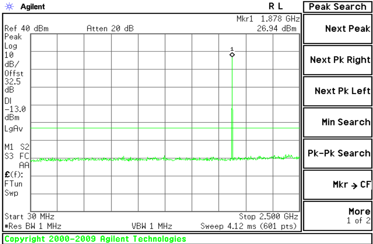
Figure 8-10: Out of Band emission at antenna terminals – GSM CH Middle
