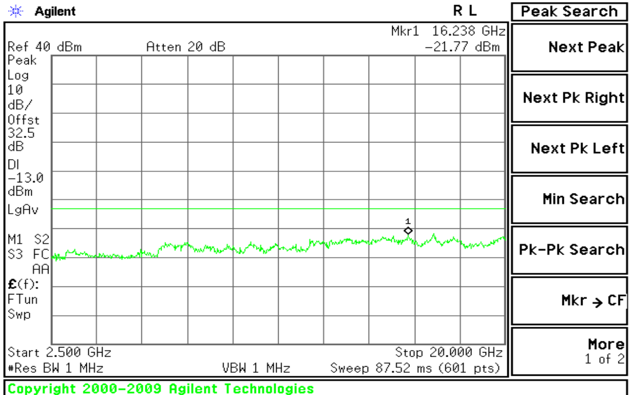
Figure 7-8: Out of Band emission at antenna terminals – GSM CH Low
