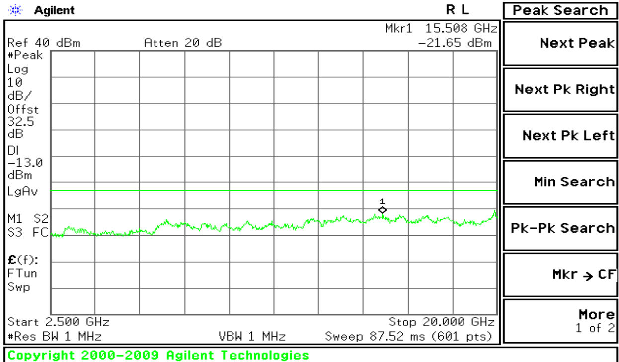
Figure 7-4: Out of Band emission at antenna terminals – GSM CH Mid
