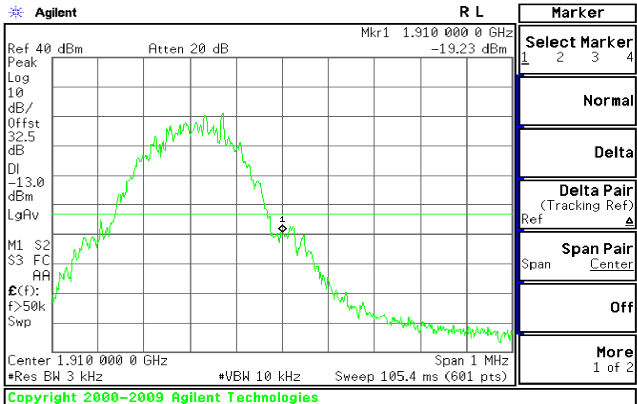
Figure 10-4: Band Edge emissions – GPRS CH High
