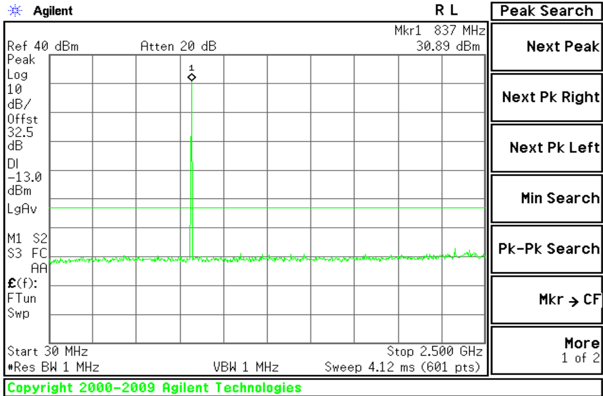
Figure 7-10: Out of Band emission at antenna terminals – GSM CH Middle
