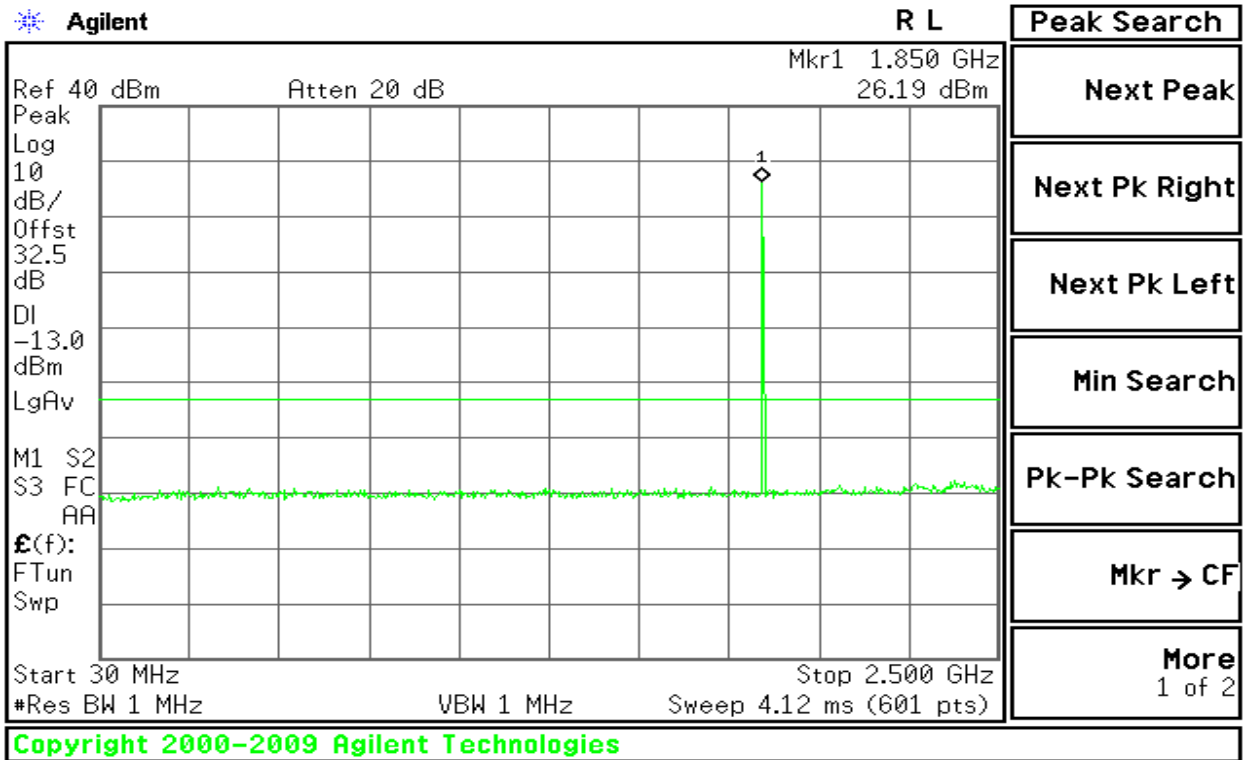
Figure 8-8: Out of Band emission at antenna terminals – GSM CH Low
