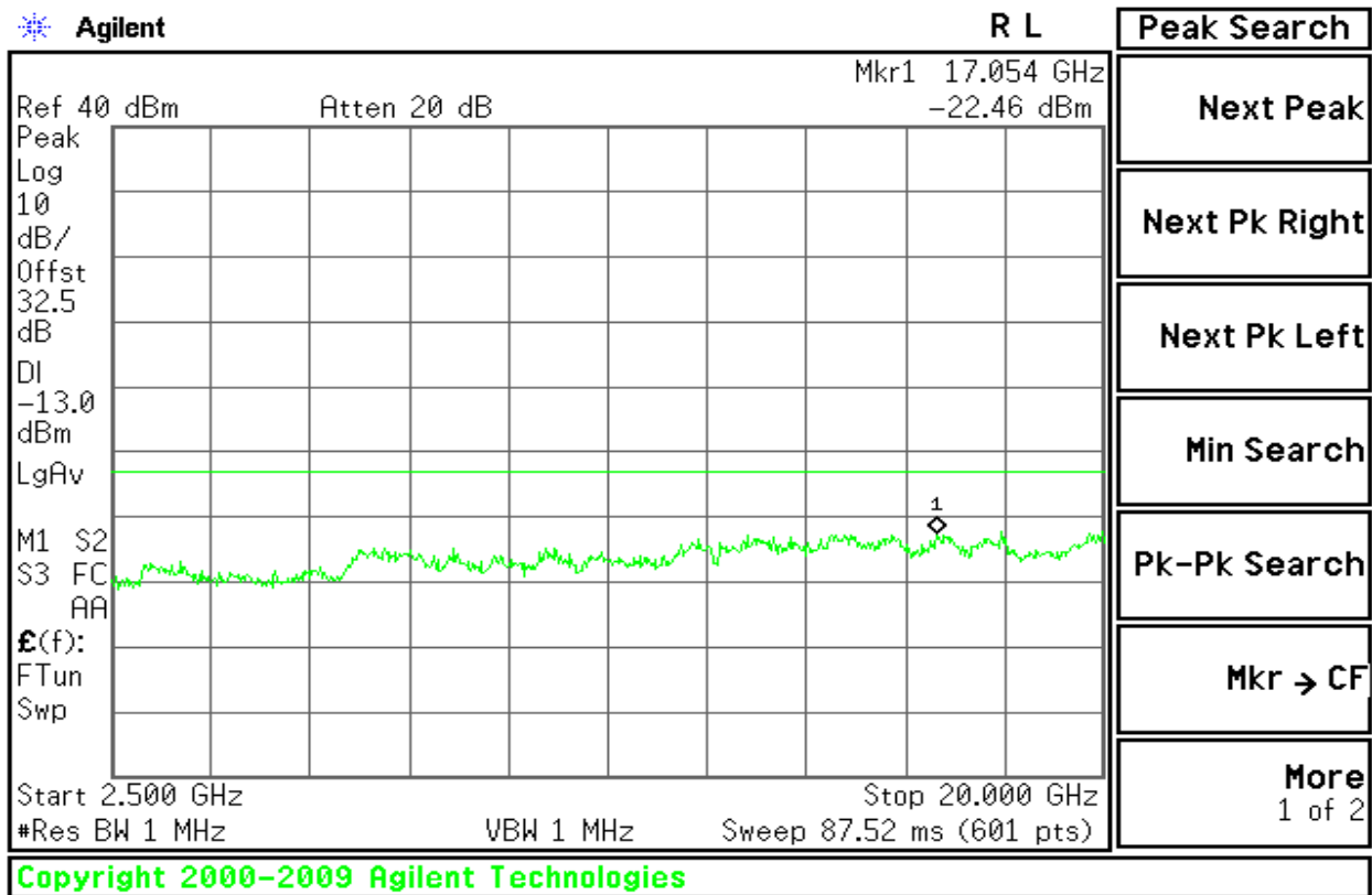
Figure 7-10: Out of Band emission at antenna terminals – GSM CH Middle
