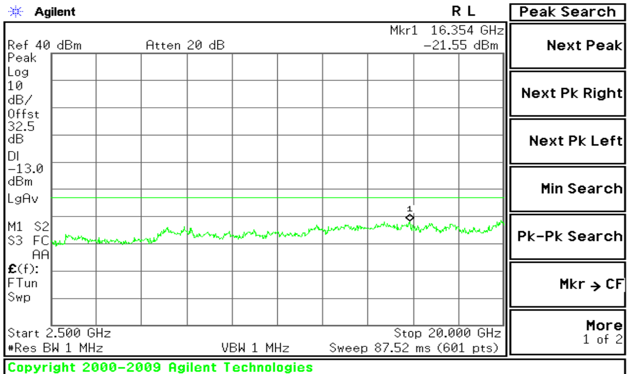
Figure 8-12: Out of Band emission at antenna terminals – GSM CH High
