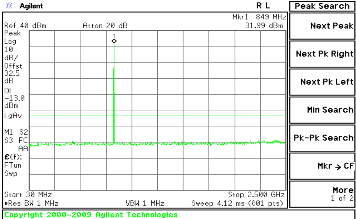
Figure 7-12: Out of Band emission at antenna terminals – GSM CH High
