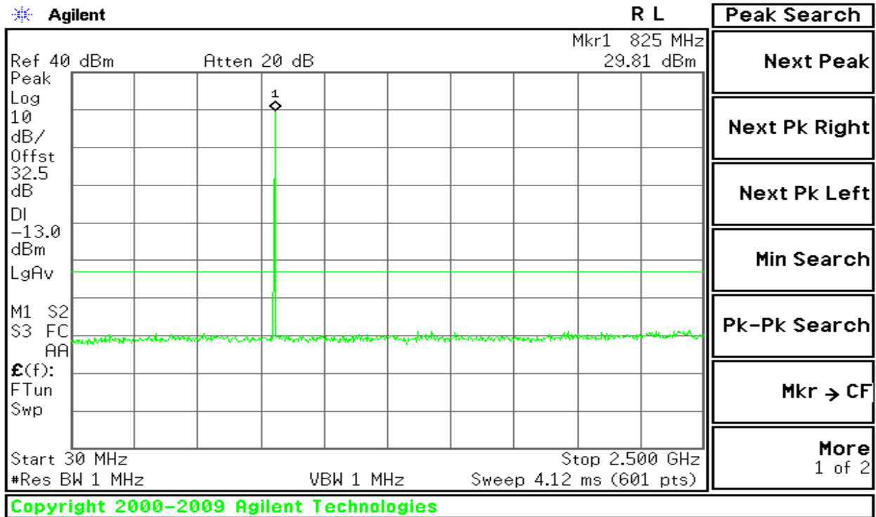
Figure 7-8: Out of Band emission at antenna terminals – GSM CH Low
