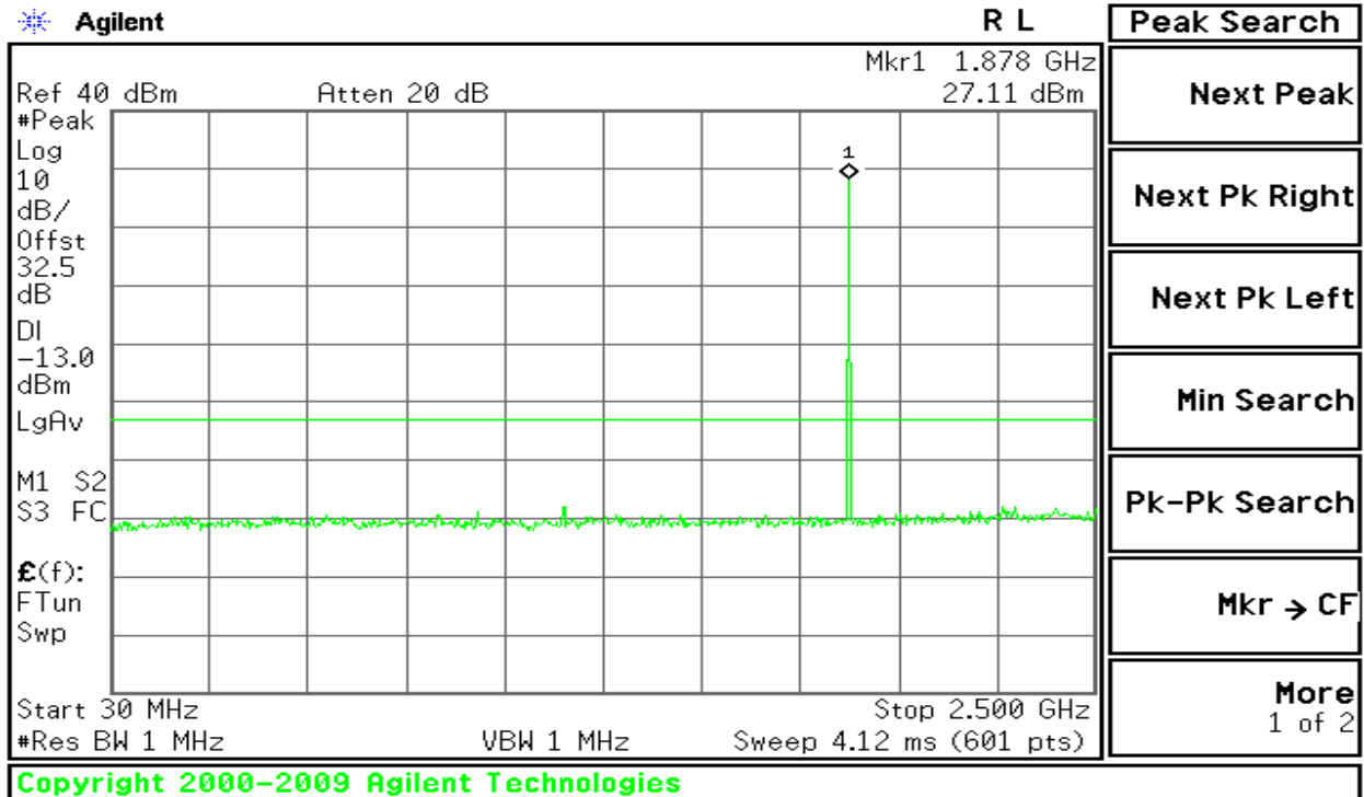
Figure 8-4: Out of Band emission at antenna terminals – GSM CH Mid
