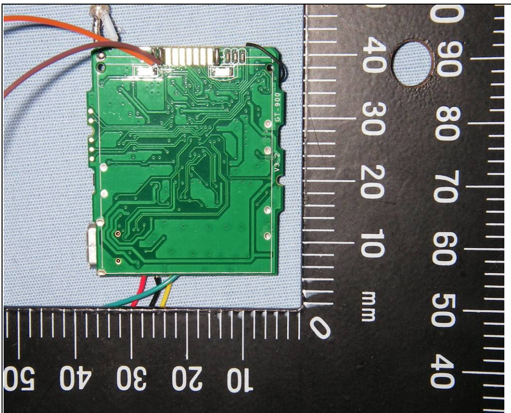
PCB1, back:
