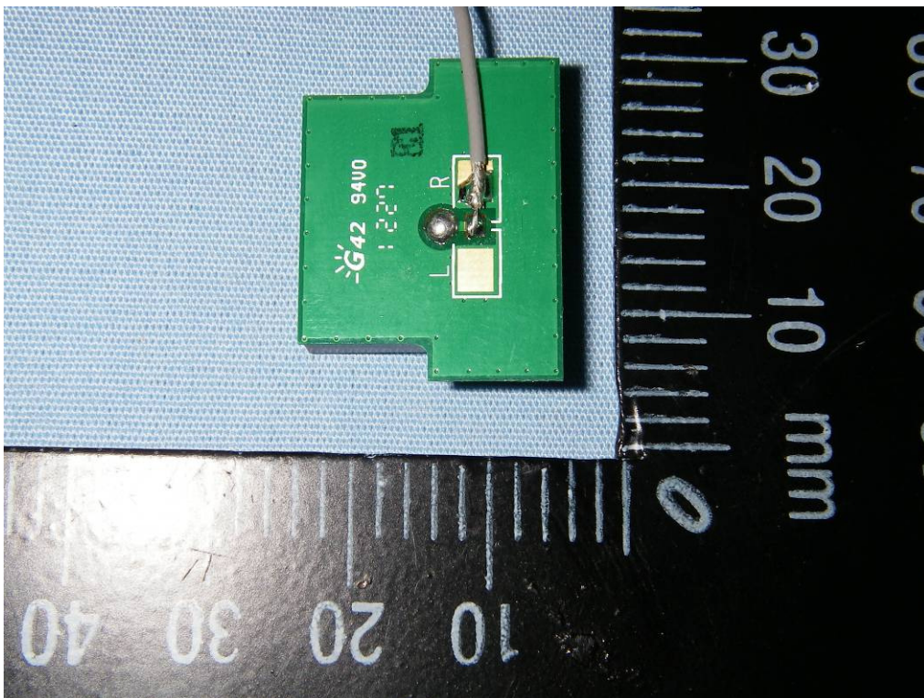
PCB2, back
