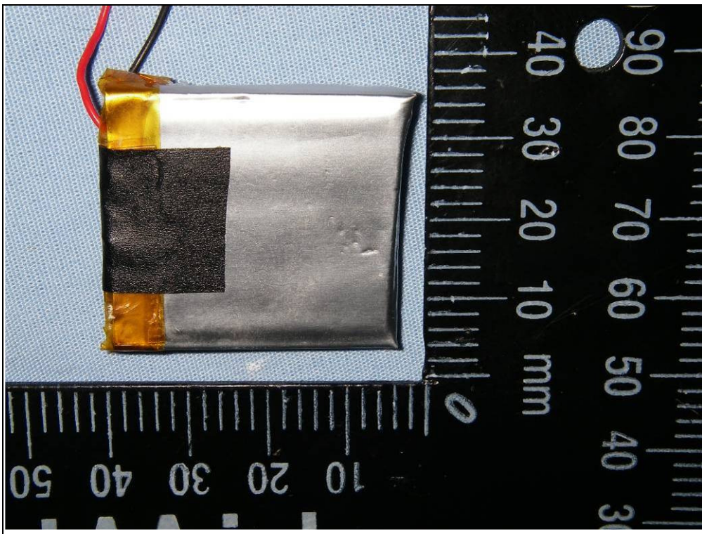
Battery, back:
