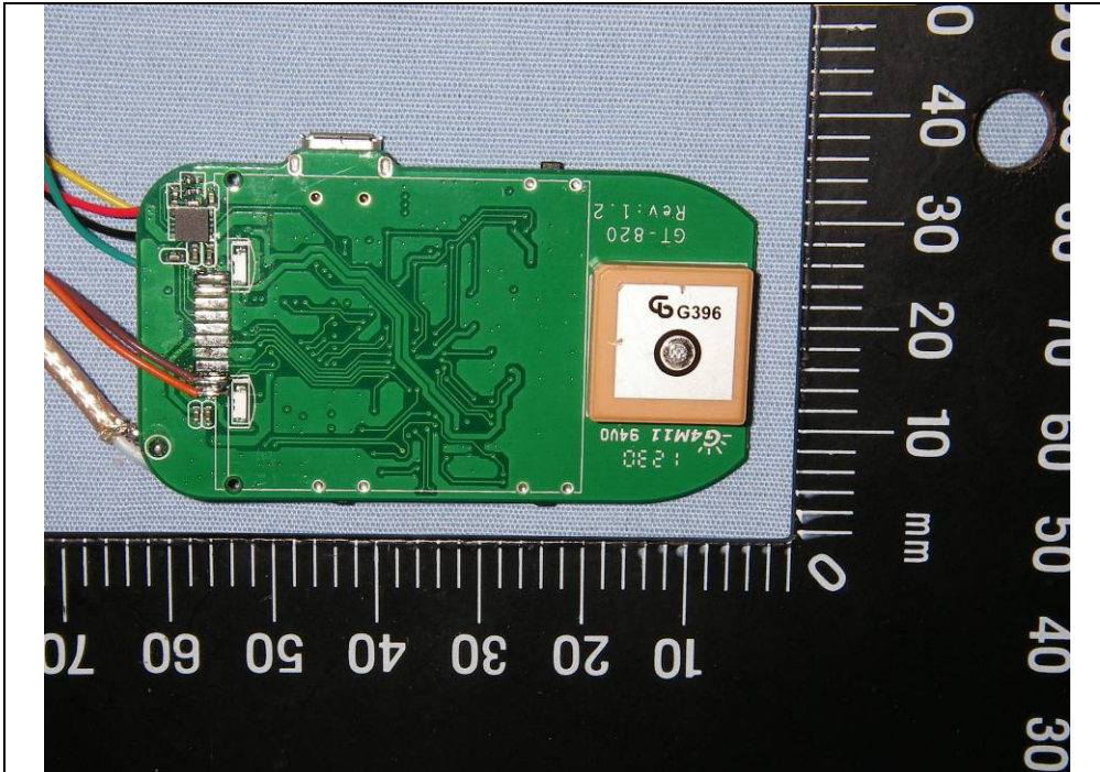
PCB, back:
