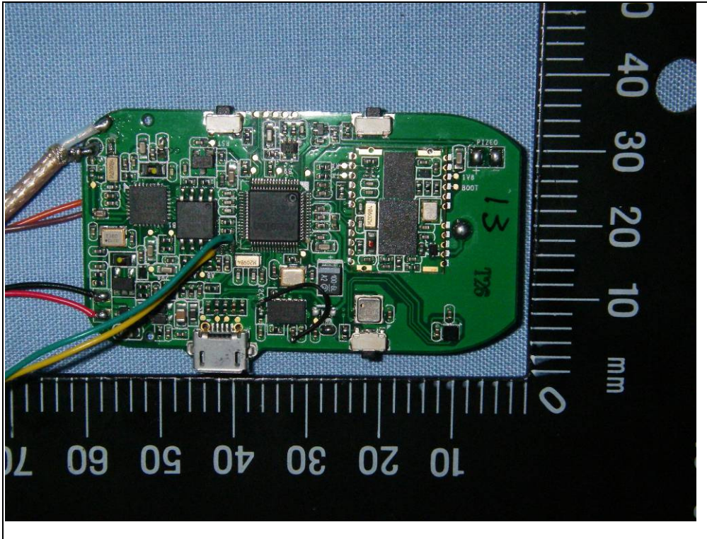
PCB, front:
