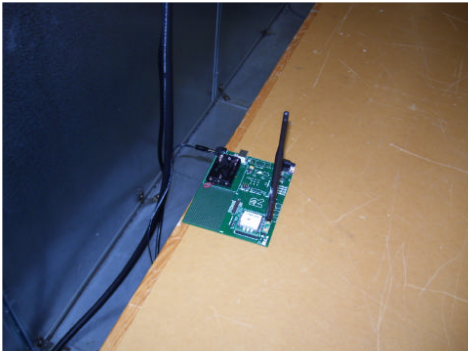
Figure 15 Conducted Emissions setup with evaluation board
