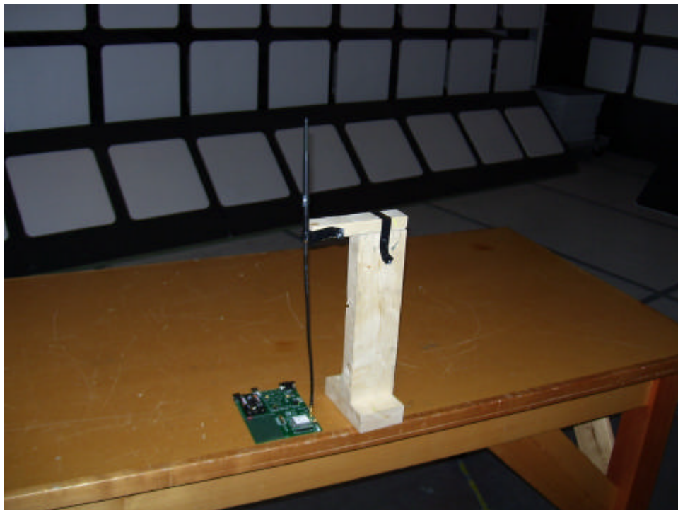
Figure 17 Testing with RF cable and antenna
