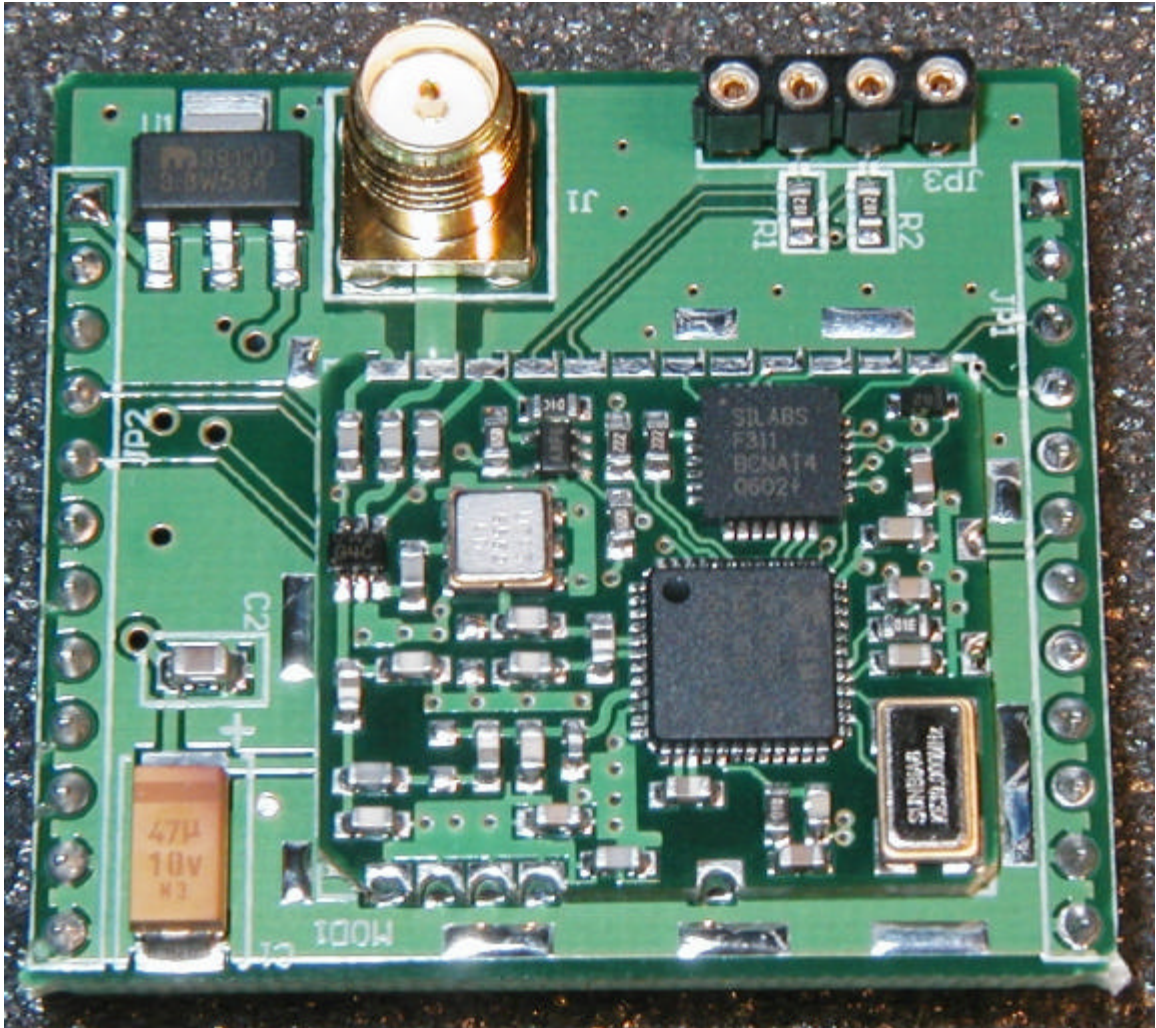
Figure 2 Module without shielding
