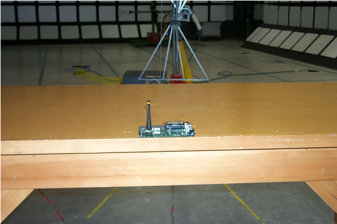
Figure 1 Test configuration
