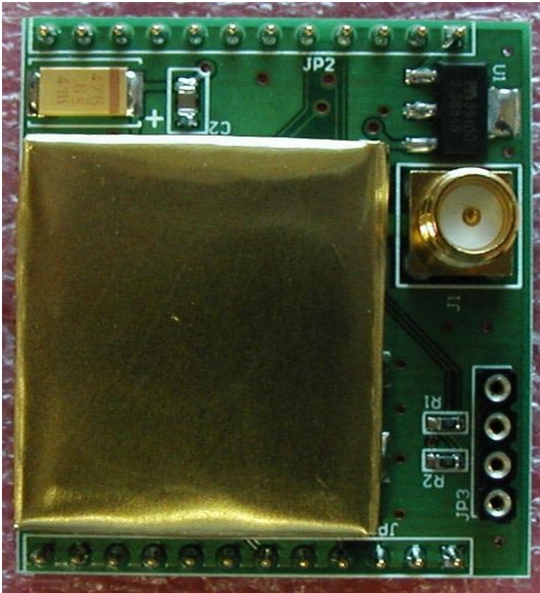
Figure 5 Top of module, with shield
