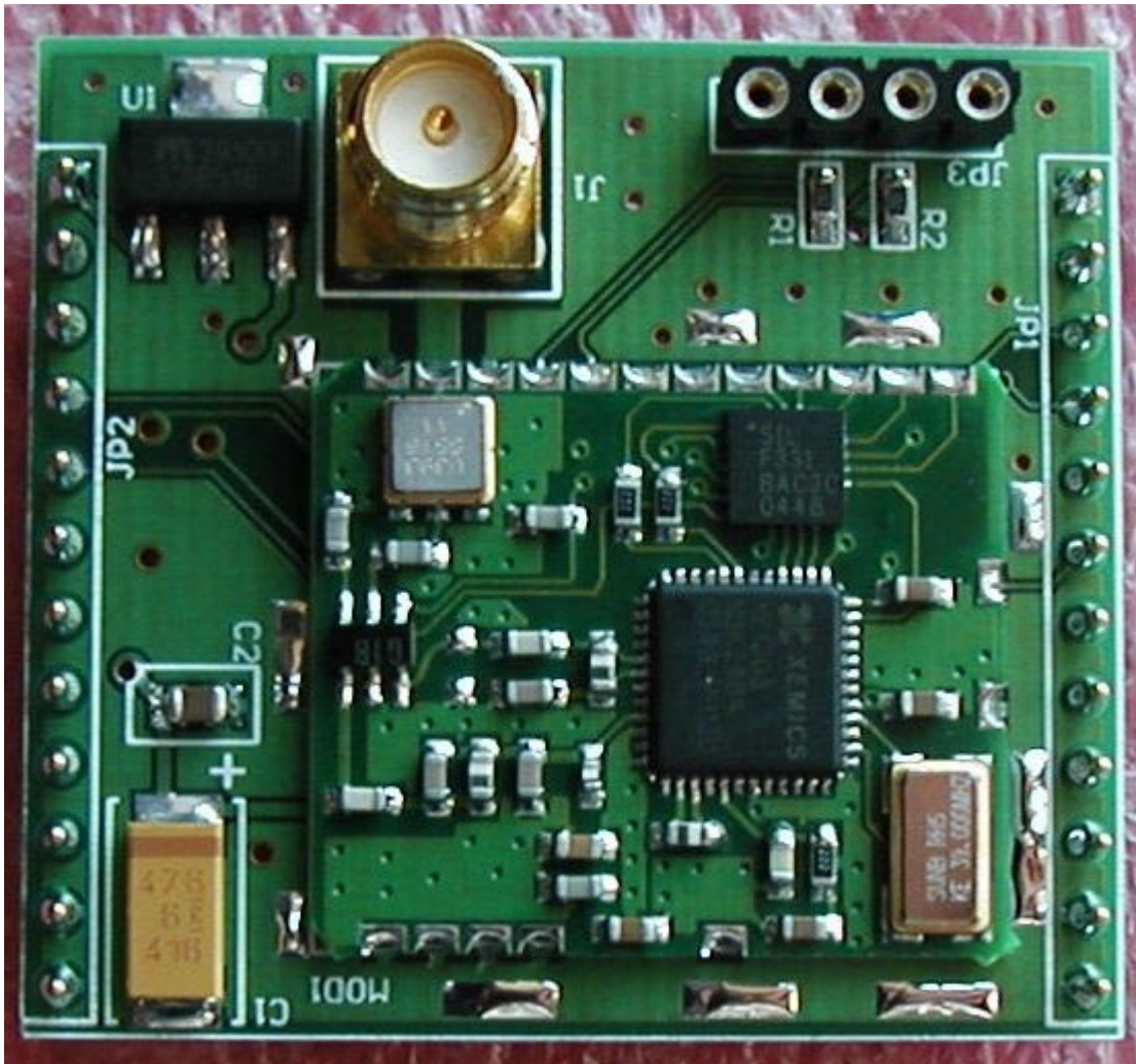
Figure 2 Top of FCC-Wi232 module, shield removed
