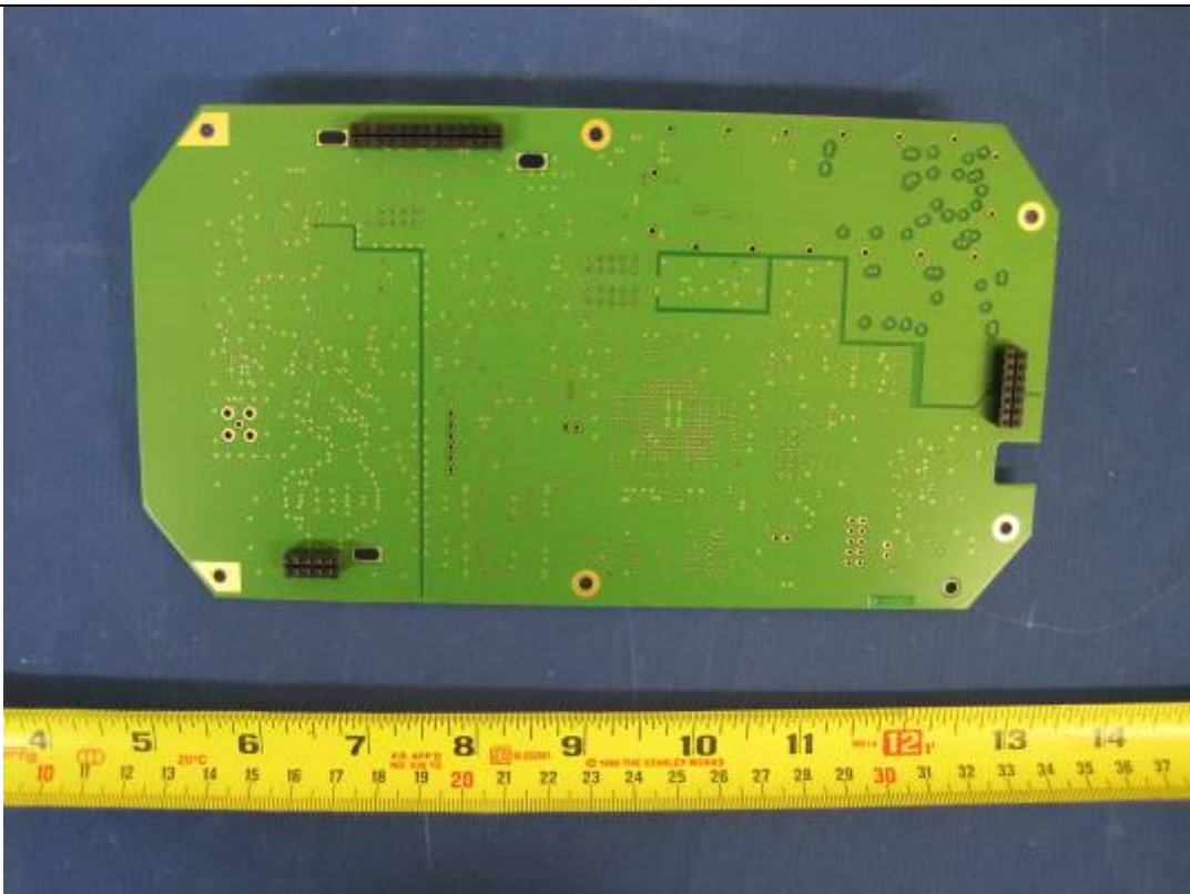
Main PCBA Solder View
