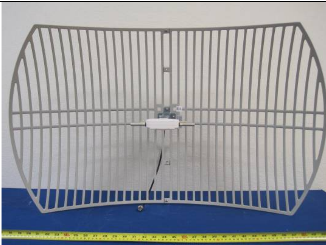
15dBi Gain Antenna – Front View
